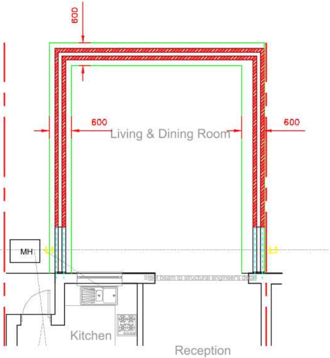
PROPOSED FOUNDATION GROUND FLOOR PLAN SCALE:-1:100
