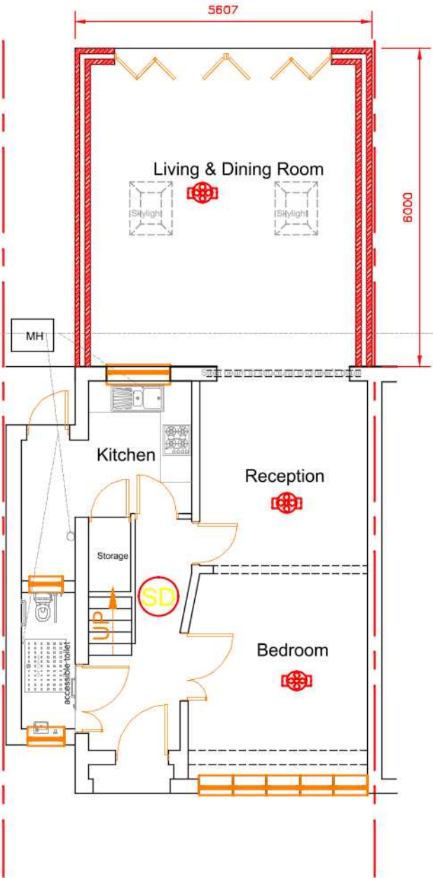
PROPOSED GROUND FLOOR PLAN SCALE:-1:100
