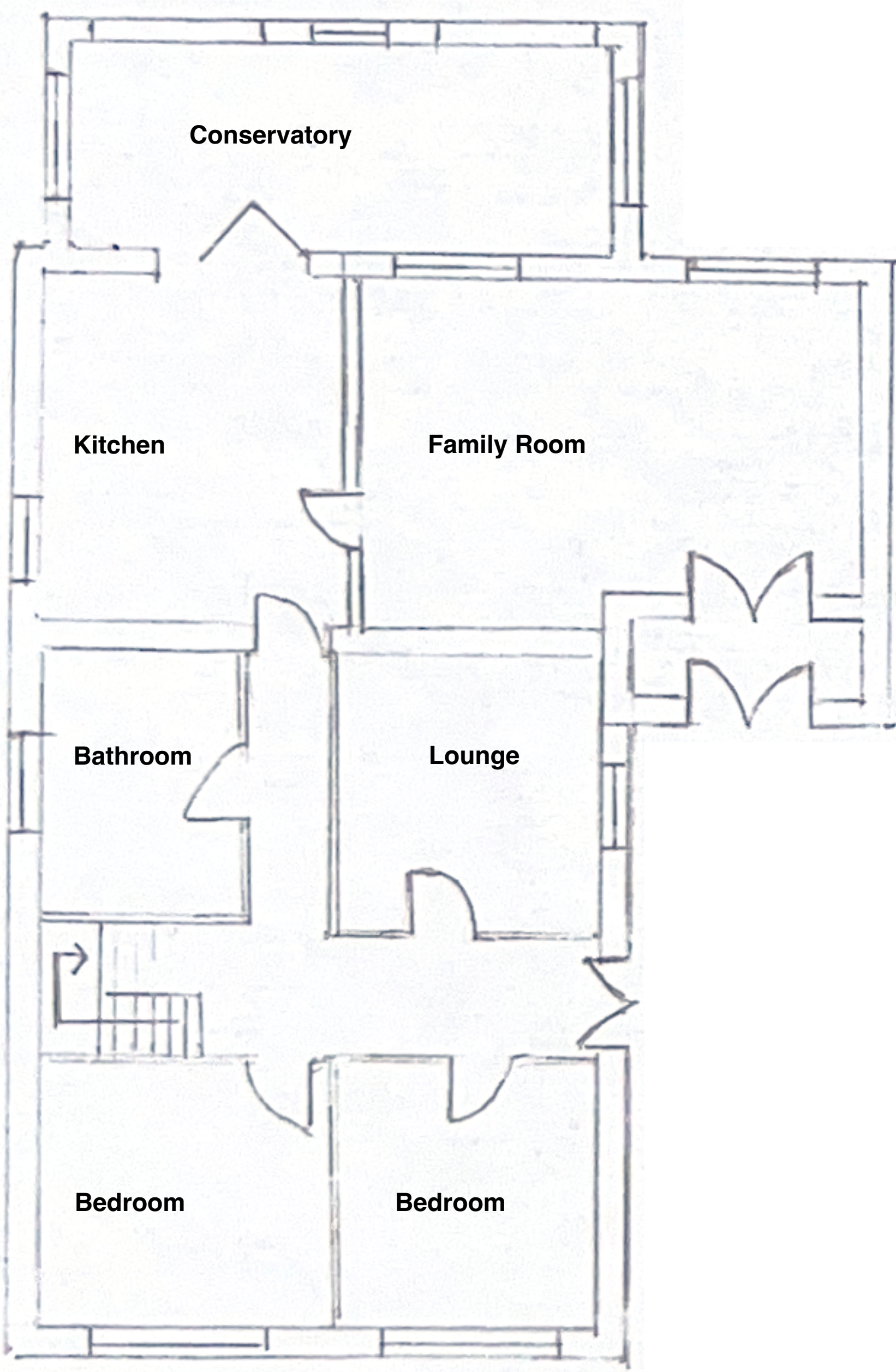
Proposed Ground Floor Plan 09.10.24
