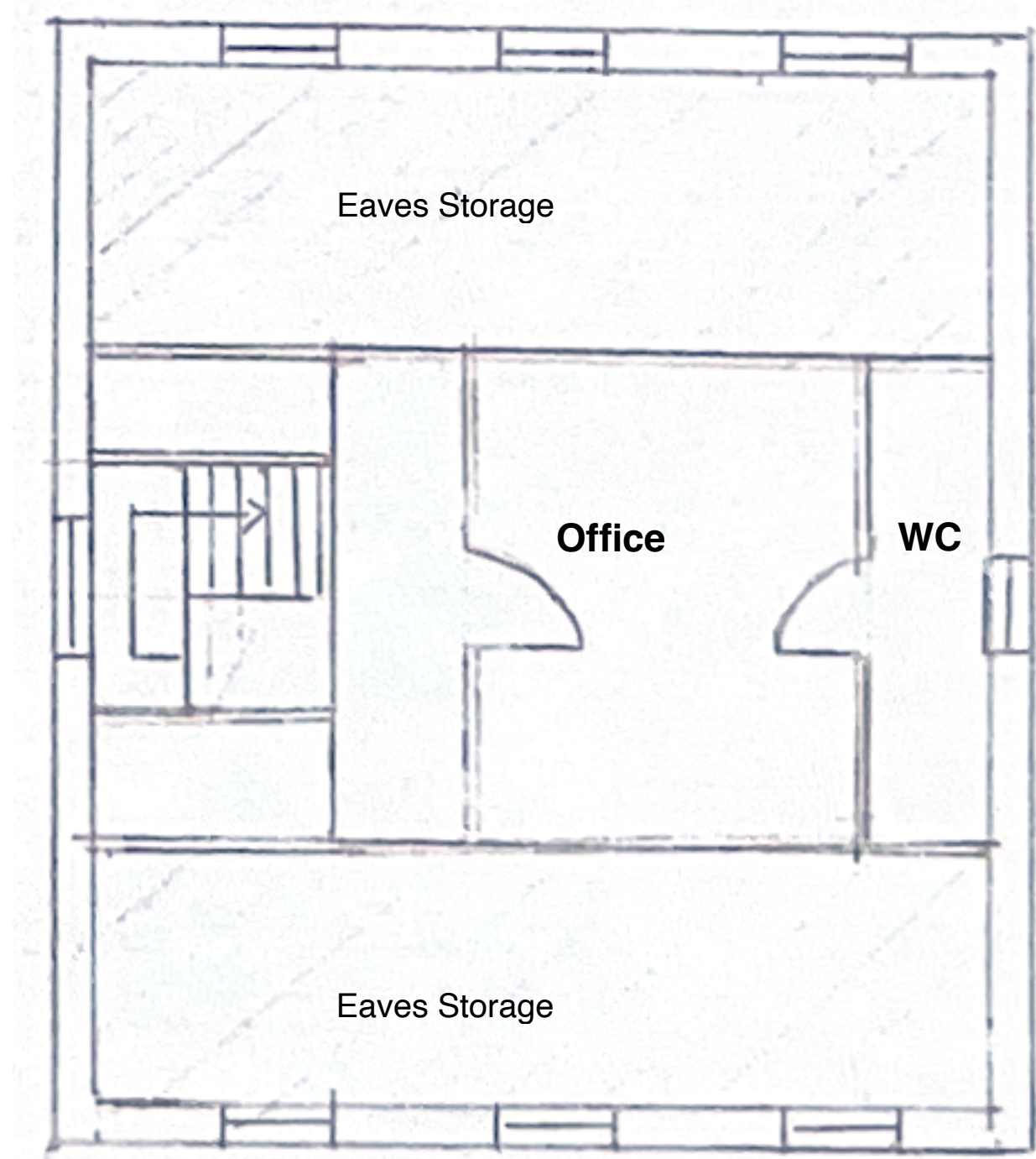
Proposed Loft Floor Plan 09.10.24
