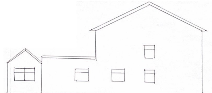
Amendment To Approved North East Elevation
