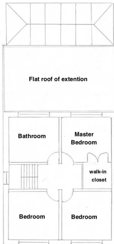
Approved First Floor Plan
