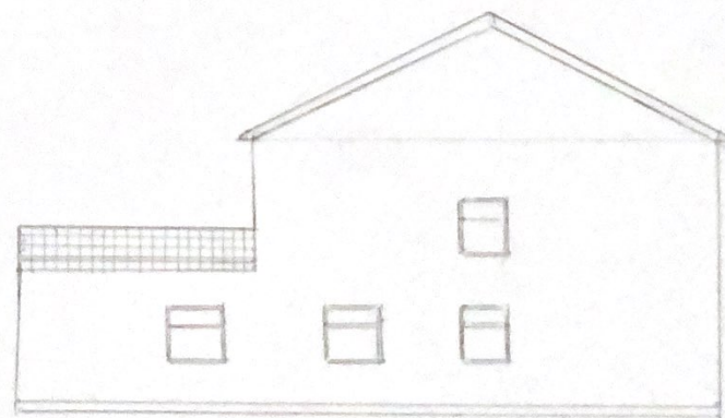
Proposed North East Elevation
