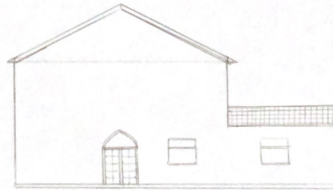
Proposed South West Elevation
