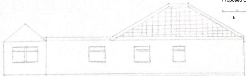
Existing North East Elevation
