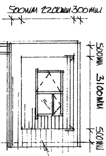
EXISTING GROUND FLOOR PLAN (1:100)
