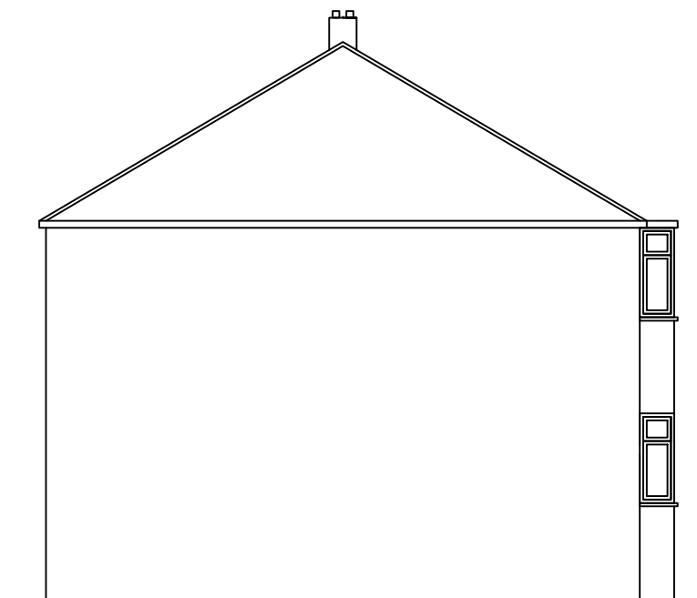
Existing South Elevation
