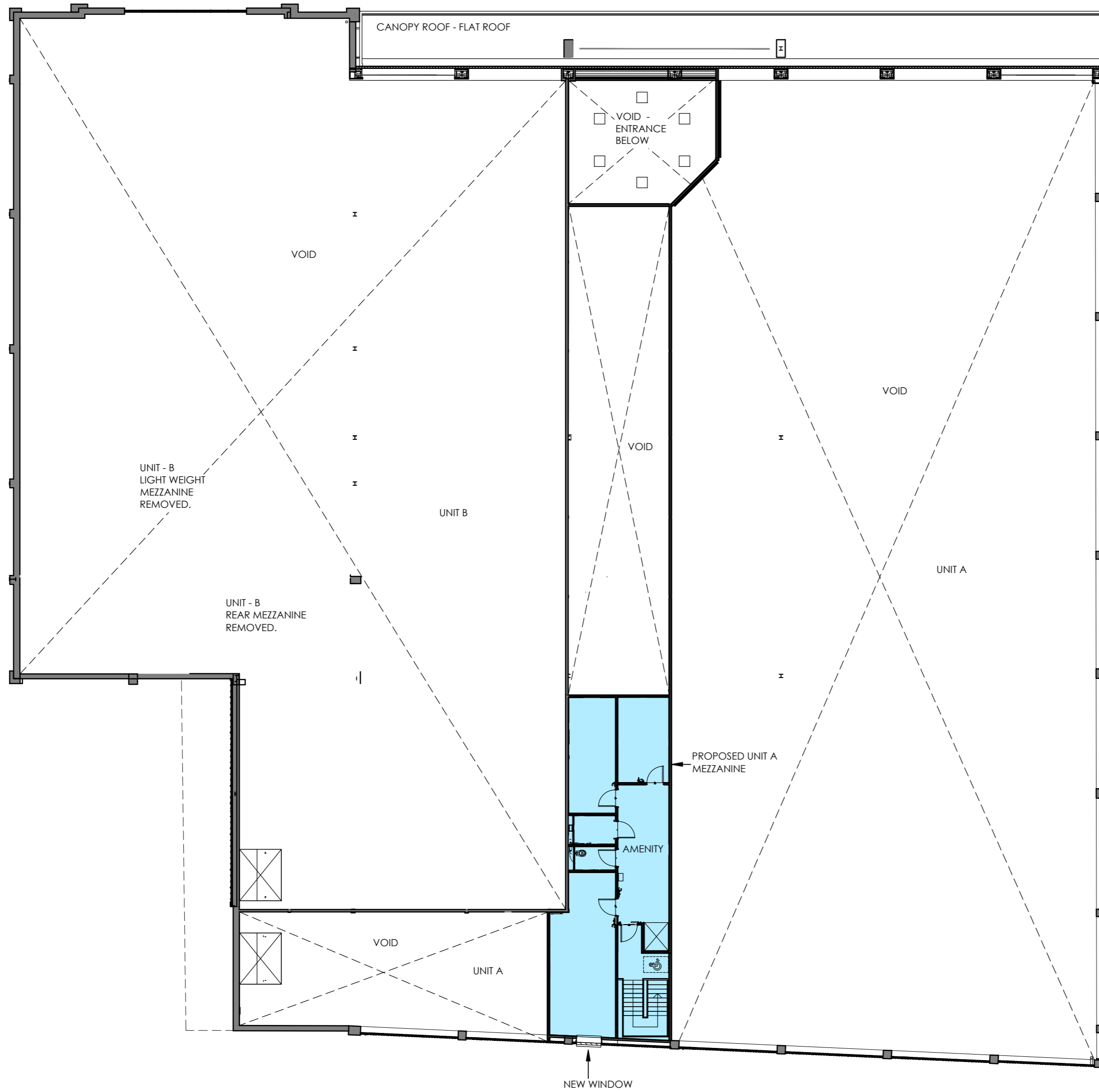
01 PROPOSED MEZZANINE FLOOR PLAN 1:200
