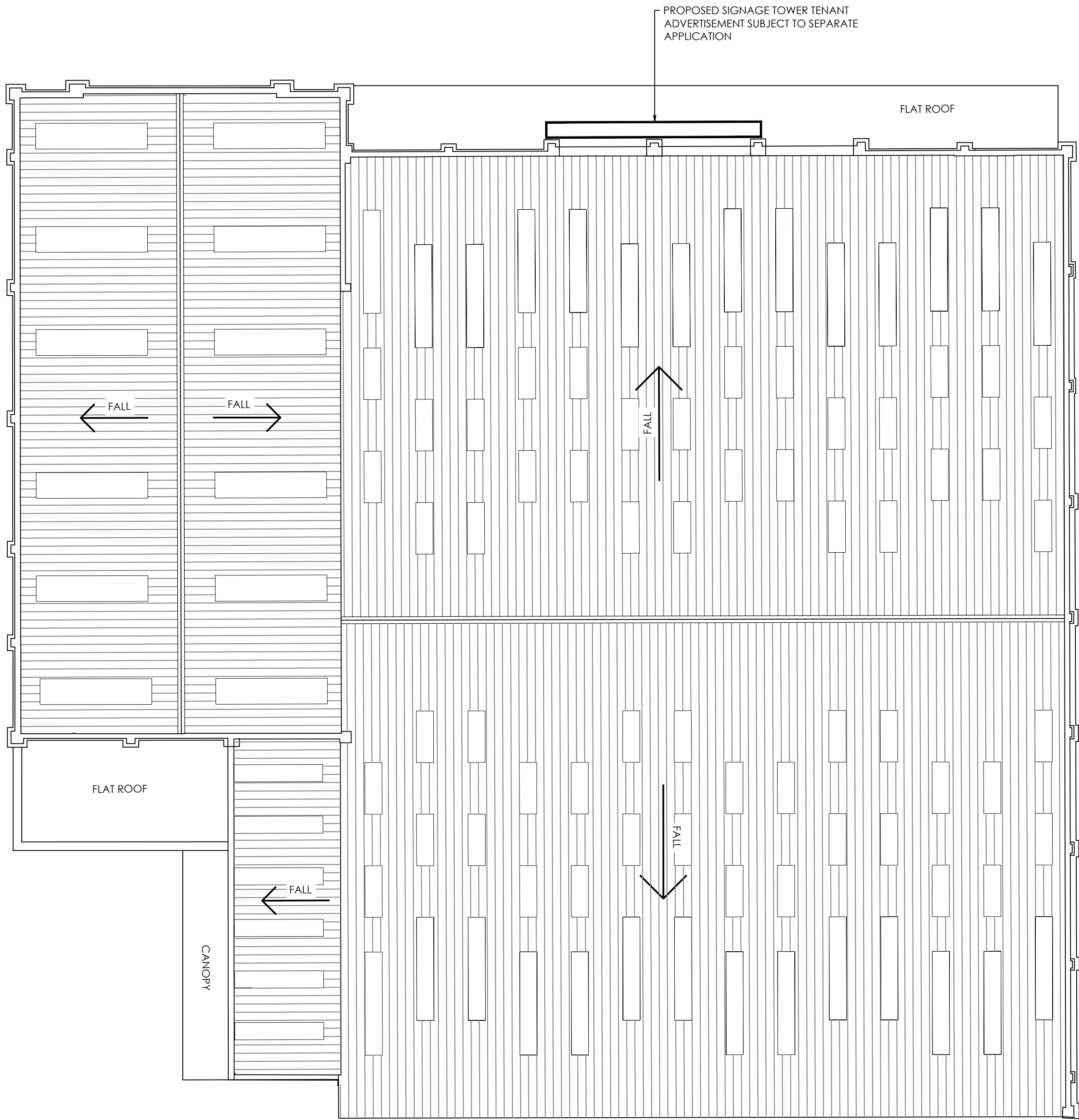
01 PROPOSED ROOF PLAN 1:200
