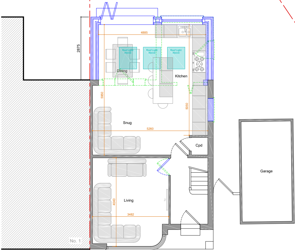
1 Proposed Ground Floor Plan
