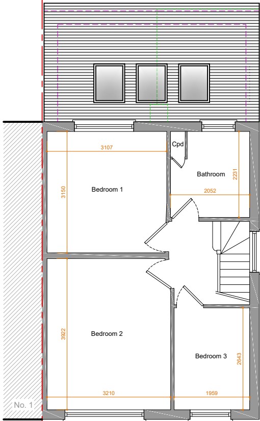
2 Proposed First Floor Plan
