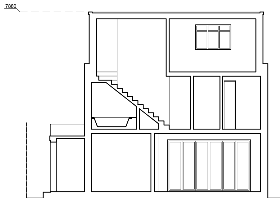
SECTION B-B' 1:100 [A2]
