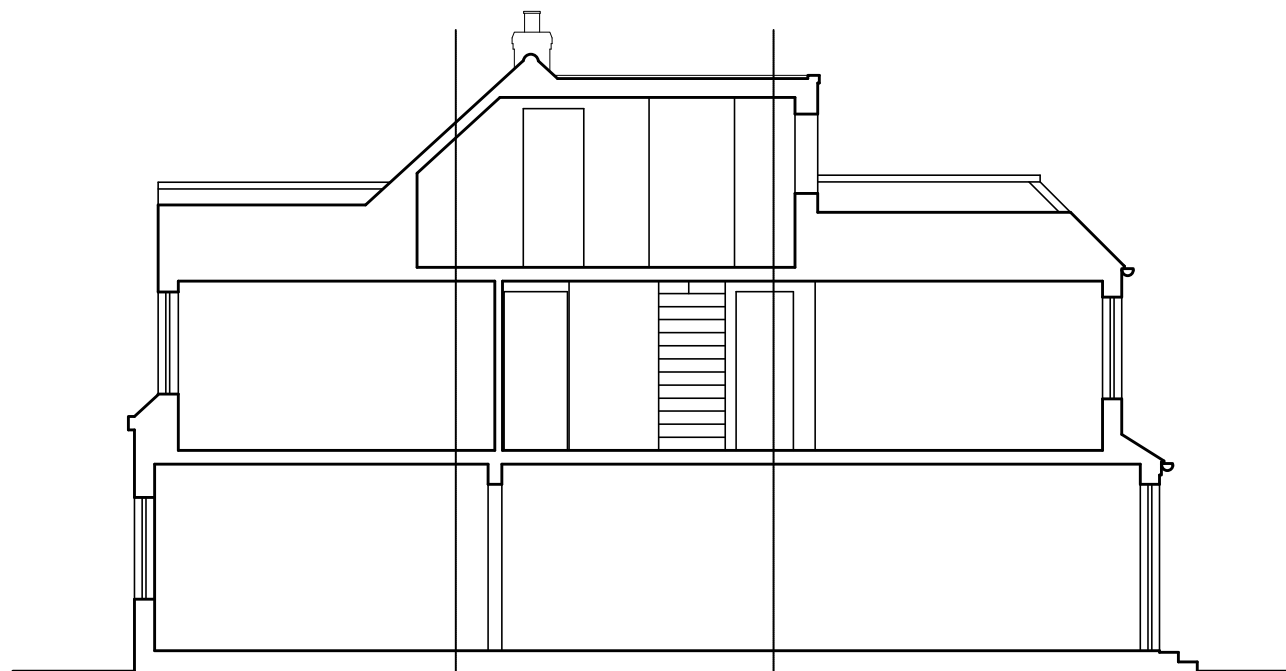
SECTION A-A' 1:100 [A2]
