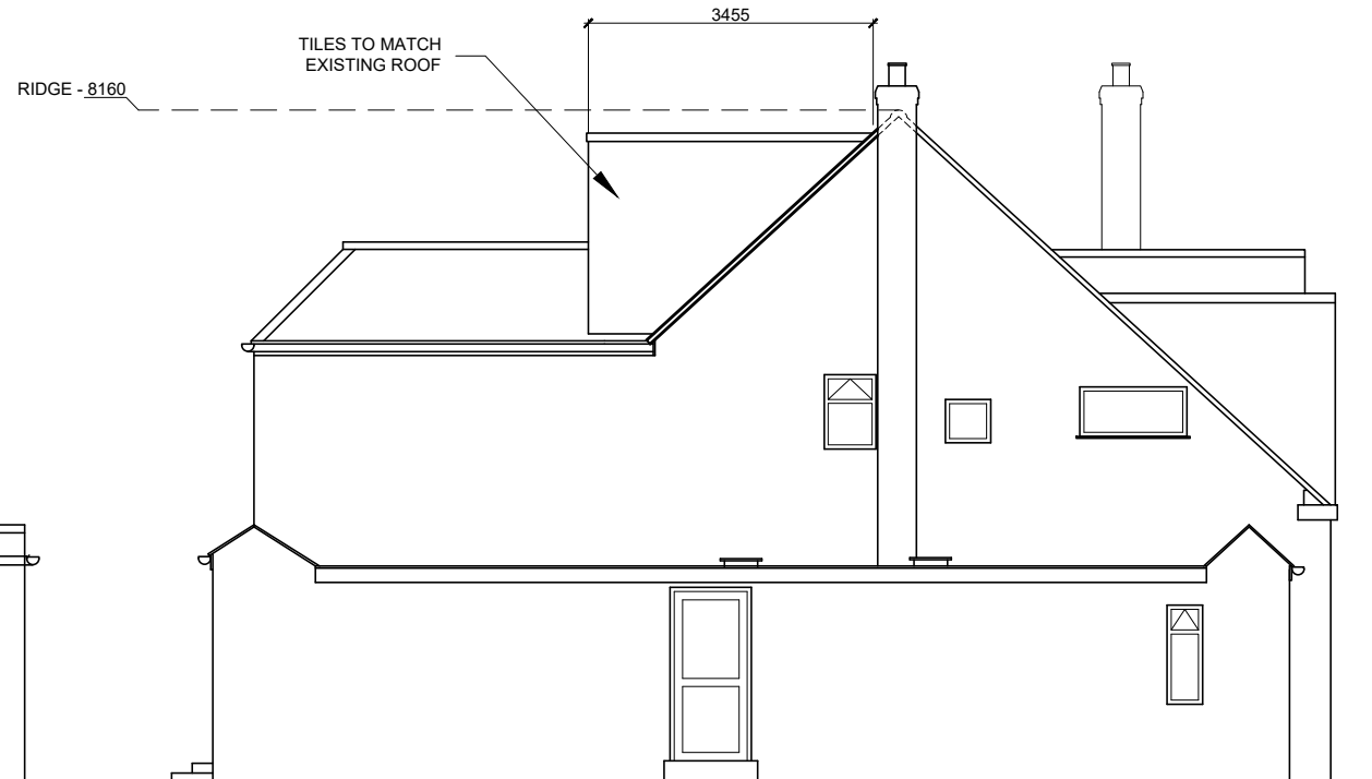
SIDE ELEVATION 1:100 [A2]
