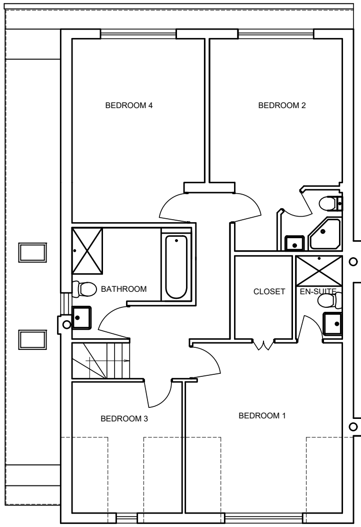
FIRST FLOOR 1:100 [A2]
