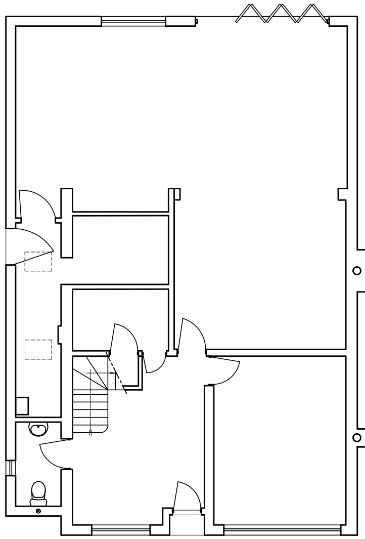
GROUND FLOOR 1:100 [A2]
