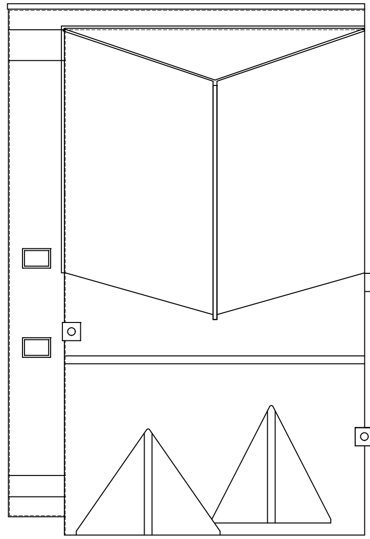
ROOF PLAN 1:100 [A2]
