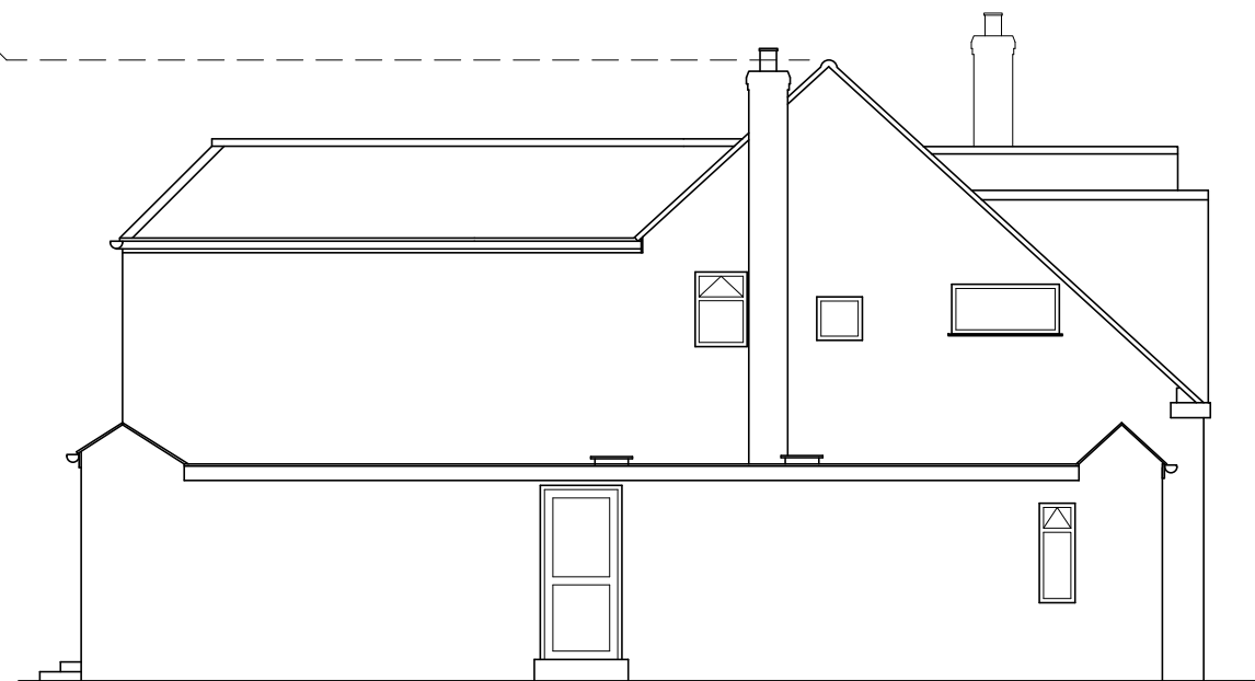
SIDE ELEVATION 1:100 [A2]
