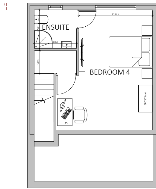
LOFT FLOOR PLAN
