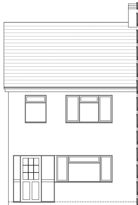
FRONT ELEVATION
