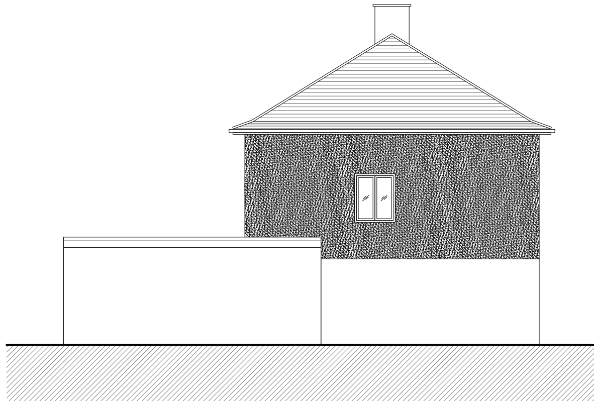
EXISTING SECTION Y-Y Scale 1:100
