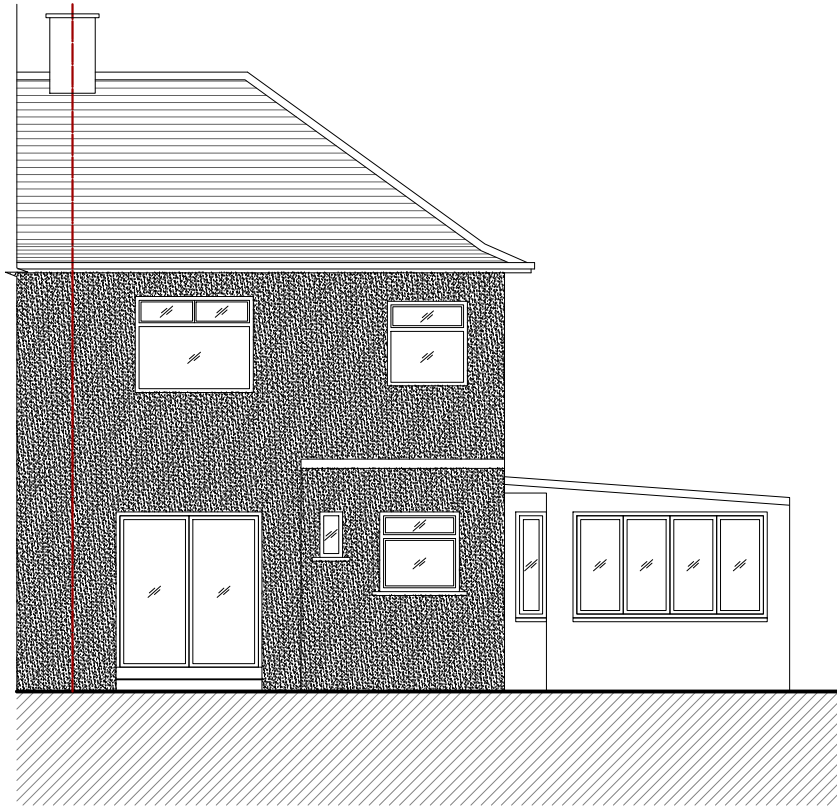
EXISTING REAR ELEVATION E3 Scale 1:100
