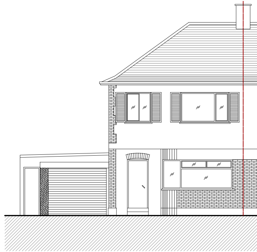
EXISTING FRONT ELEVATION E1 Scale 1:100
