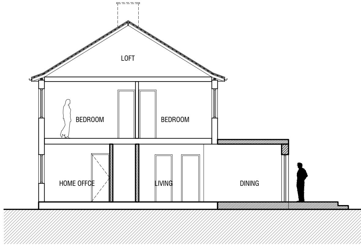
PROPOSED SECTION Y-Y Scale 1:100
