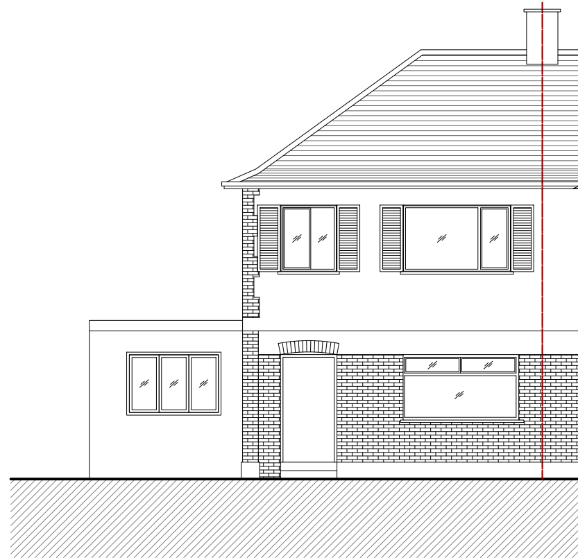
PROPOSED FRONT ELEVATION E1 Scale 1:100
