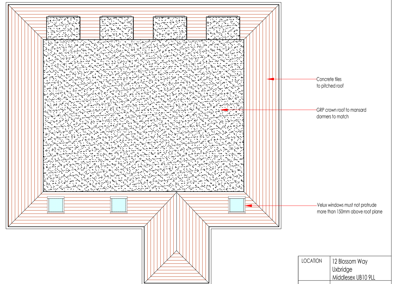
Roof Plan 1:100 at A3
