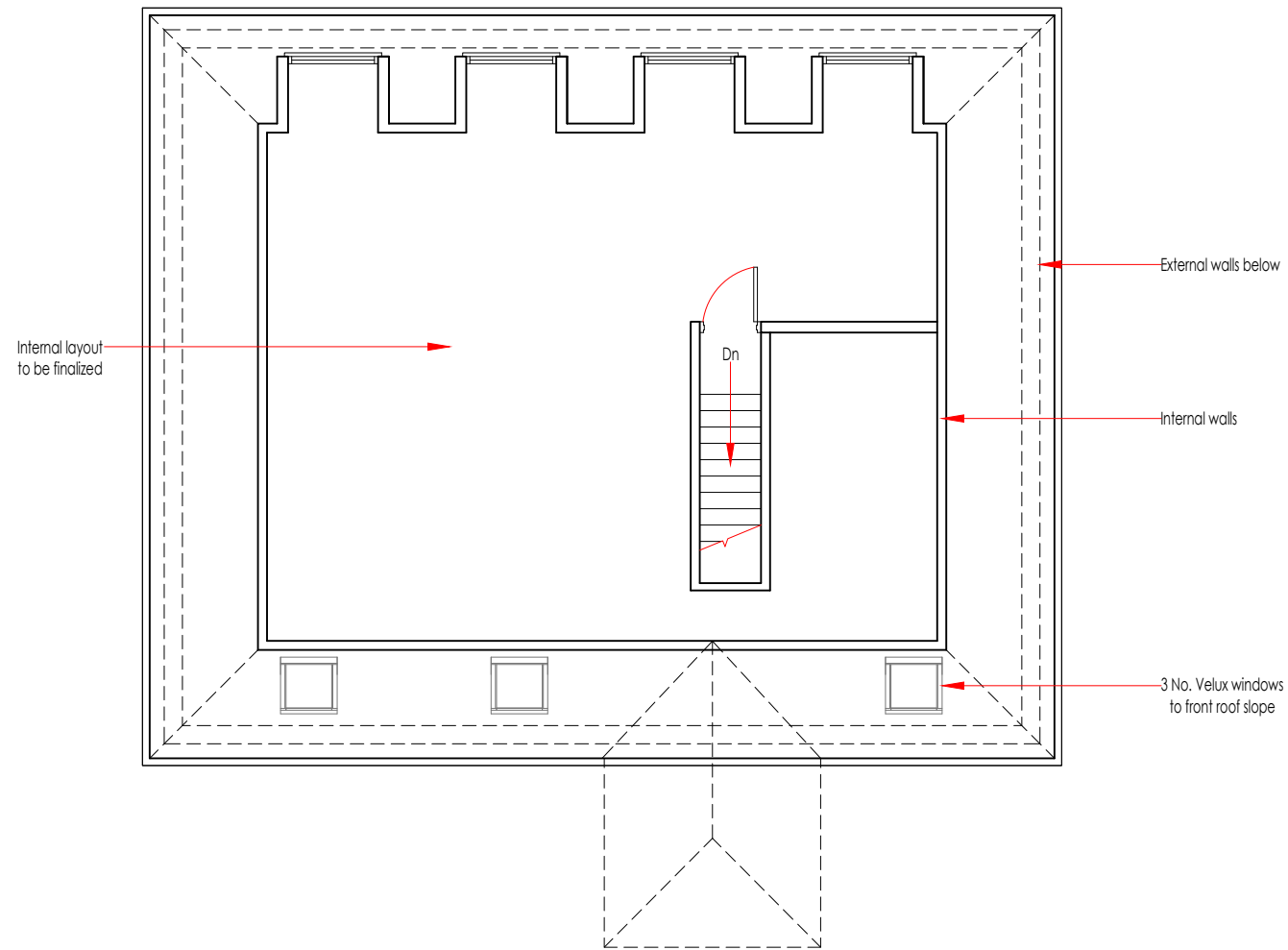
Loft Floor 1:100 at A3
