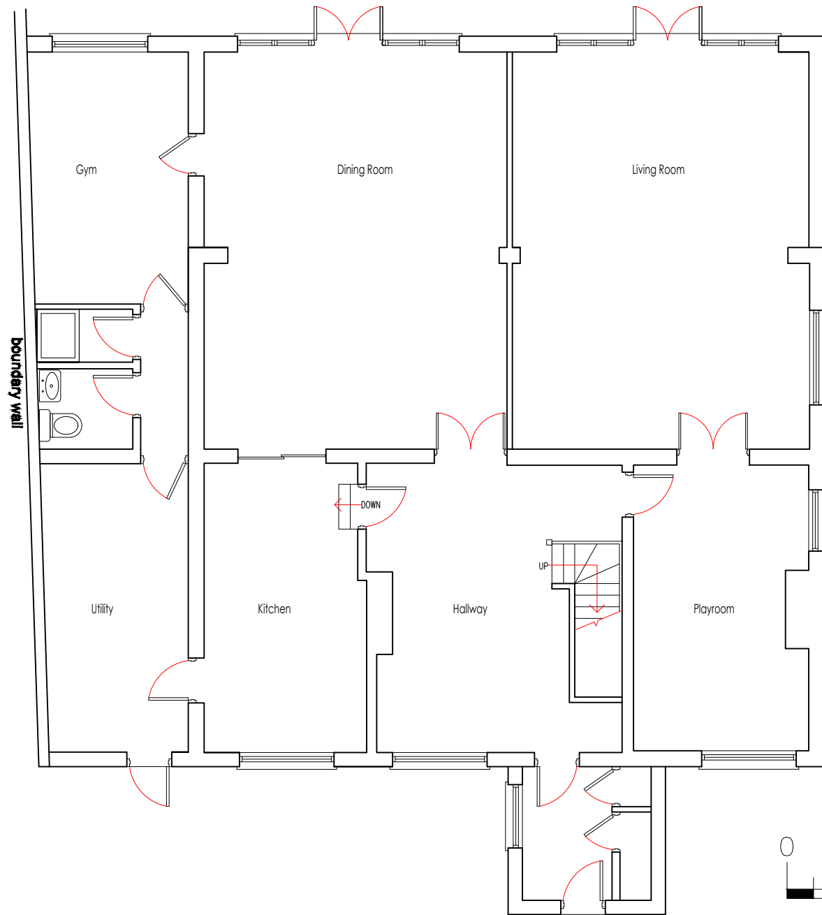
Ground Floor 1:100 at A3
