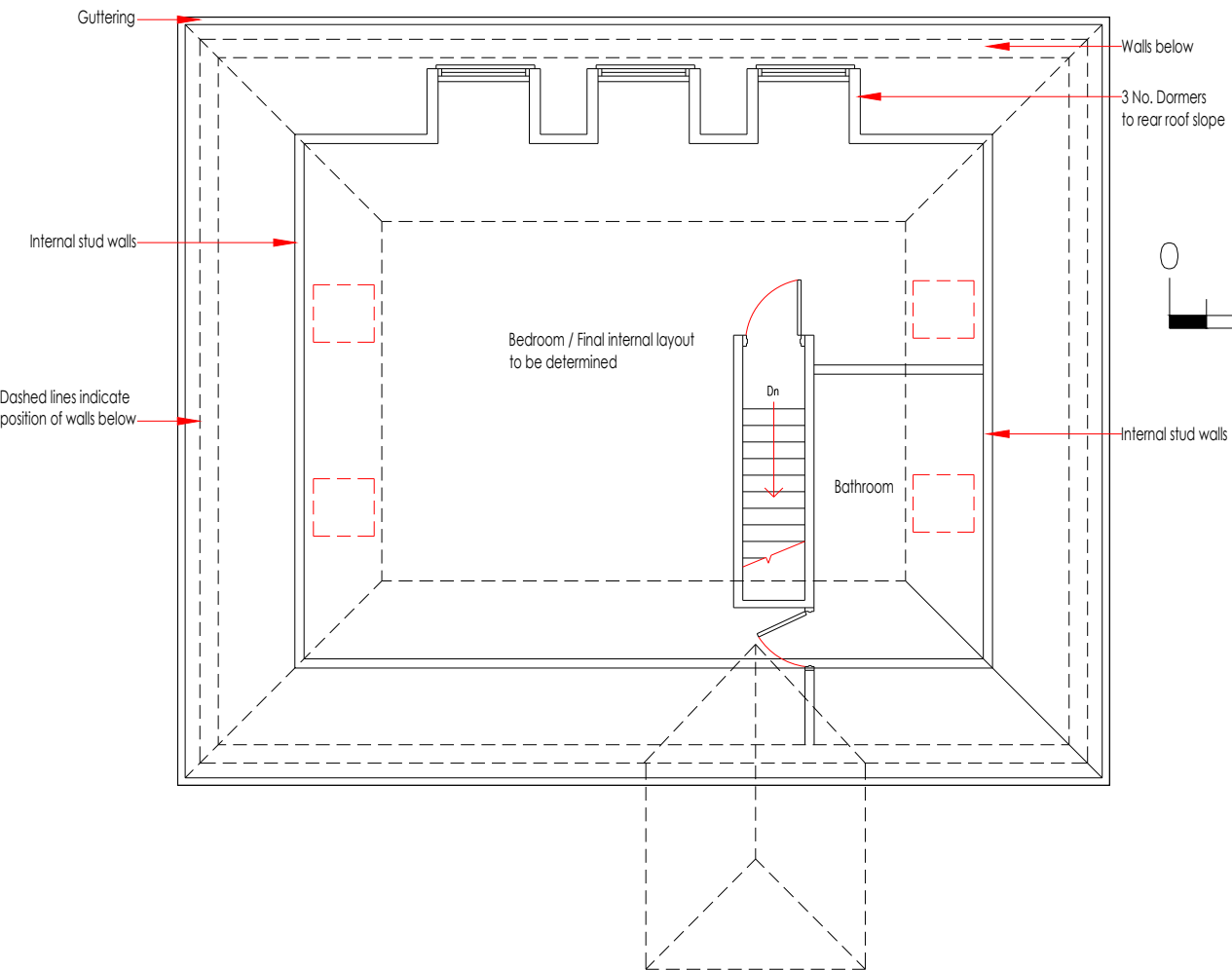
Loft Floor 1:100 at A3
