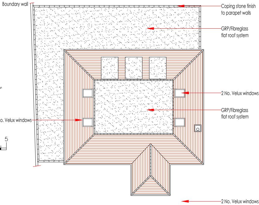
Roof Plan 1:200 at A3
