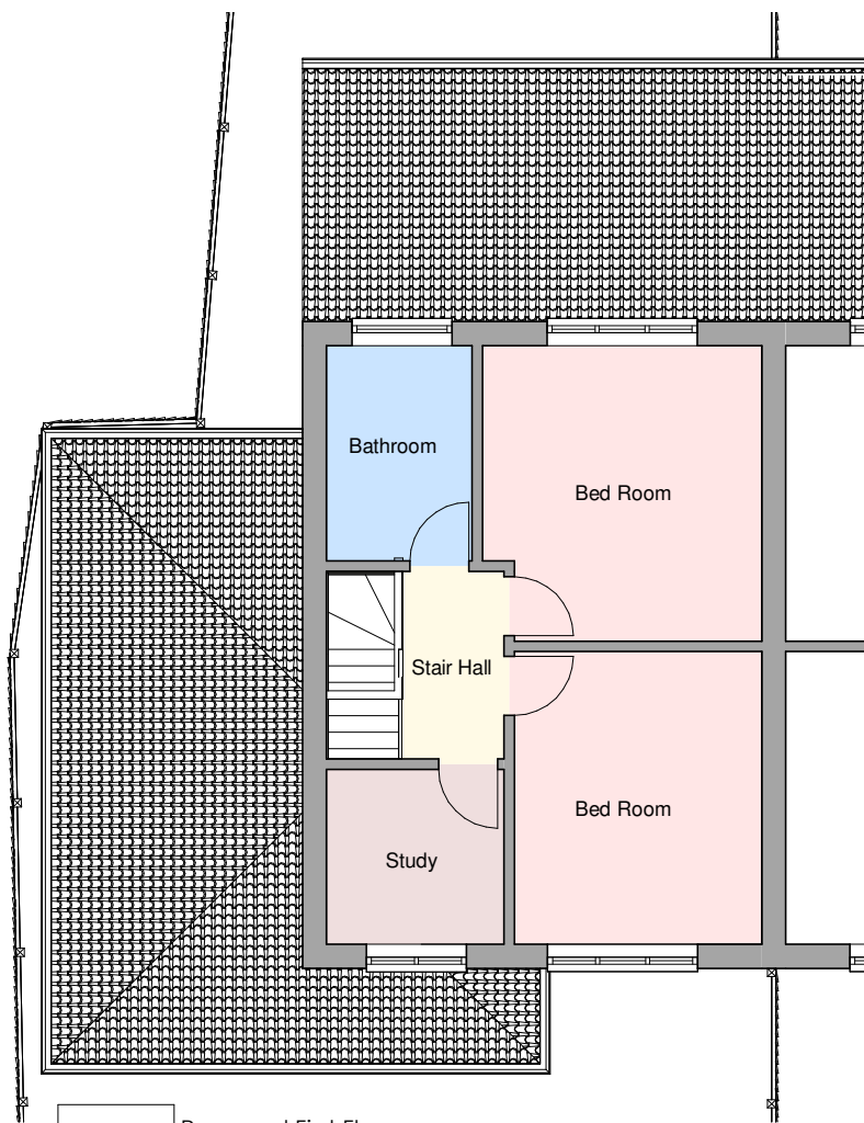
2 Proposed First Floor 2305-A-200 1 : 100
