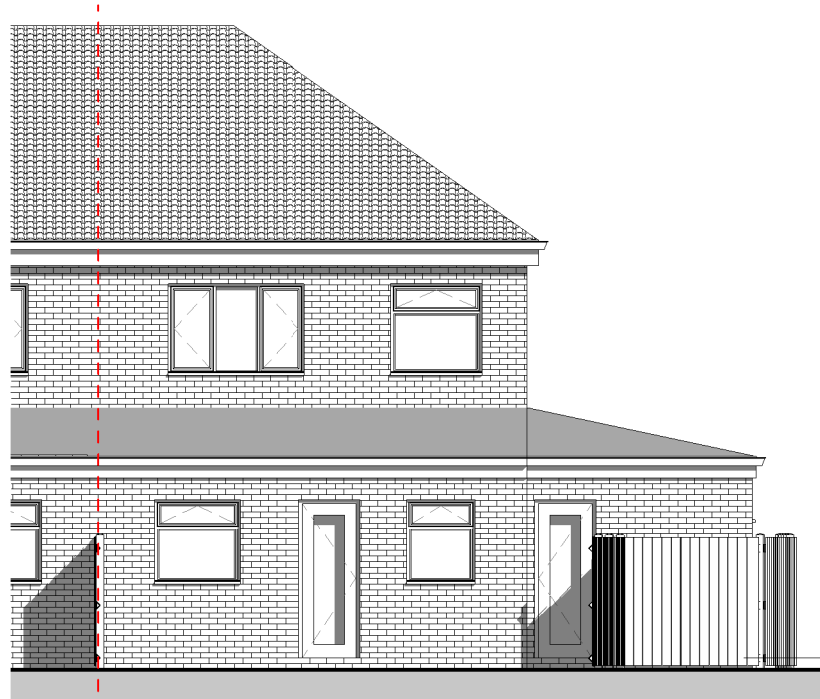
5 Proposed Rear Elevation 2305-A-200 1 : 100
