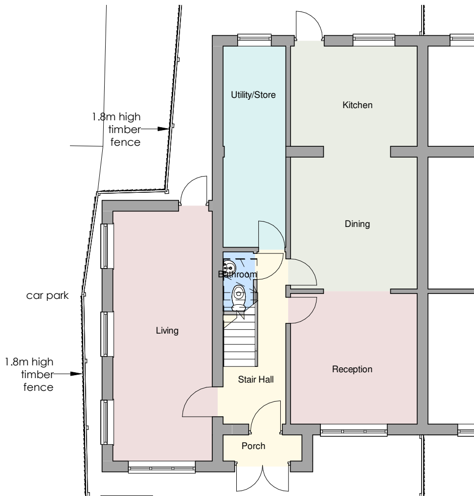
1 Proposed Ground Floor 2305-A-200 1 : 100
