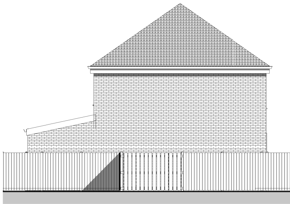
4 Existing Side Elevation (West) 2305-A-100 1 : 100
