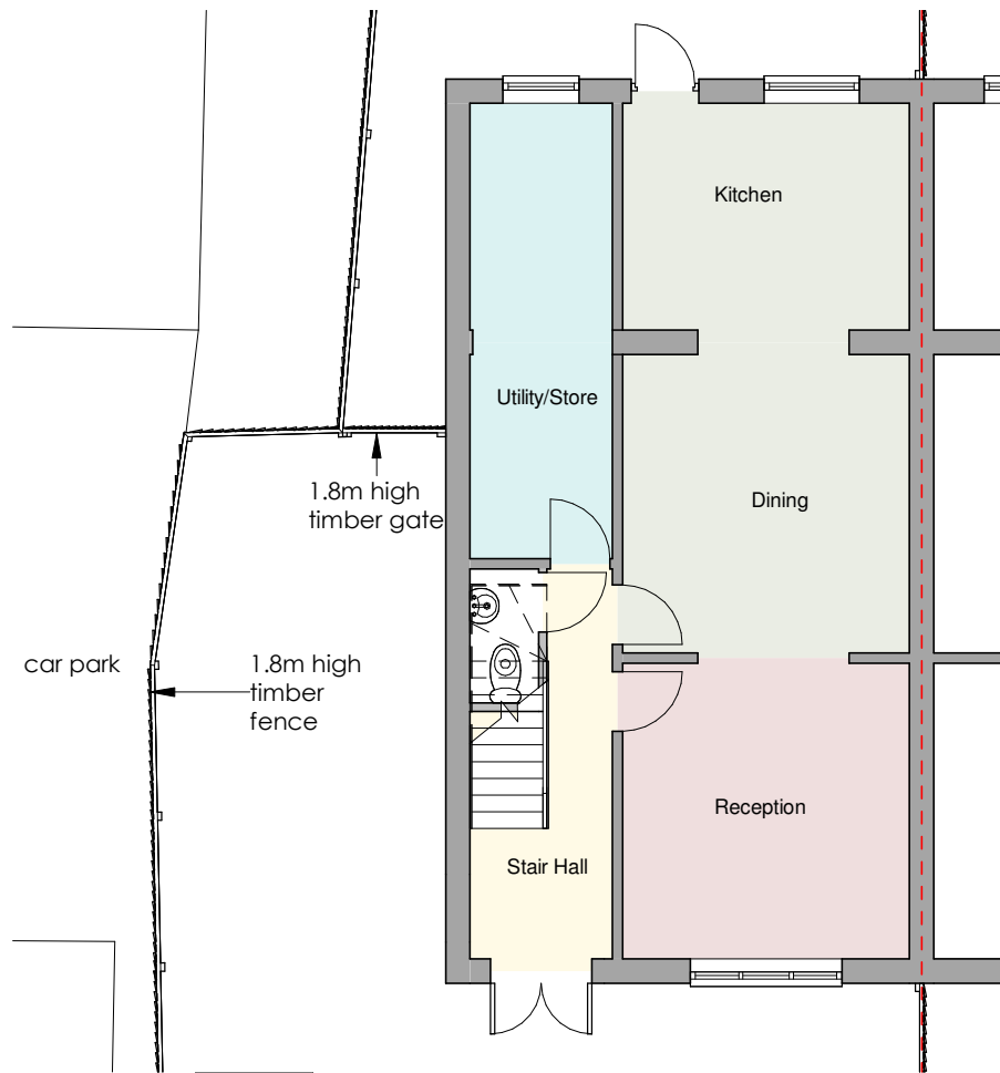
1 Existing Ground Floor 2305-A-100 1 : 100
