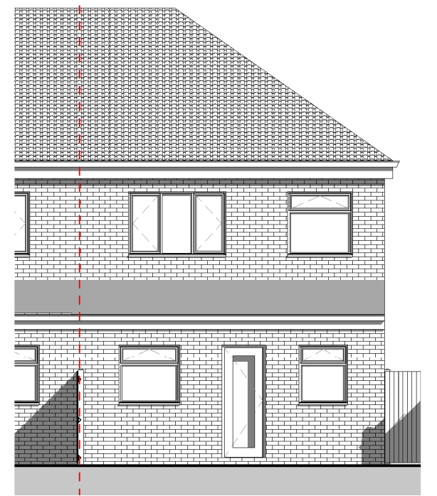
5 Existing Rear Elevation 2305-A-100 1 : 100
