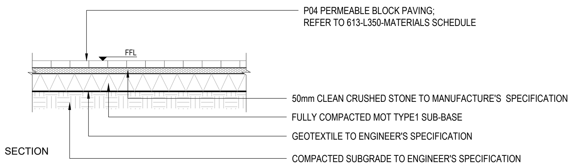
02 TYPICAL PERMEABLE BLOCK PAVING DETAIL SCALE : 1:20 @ A1
