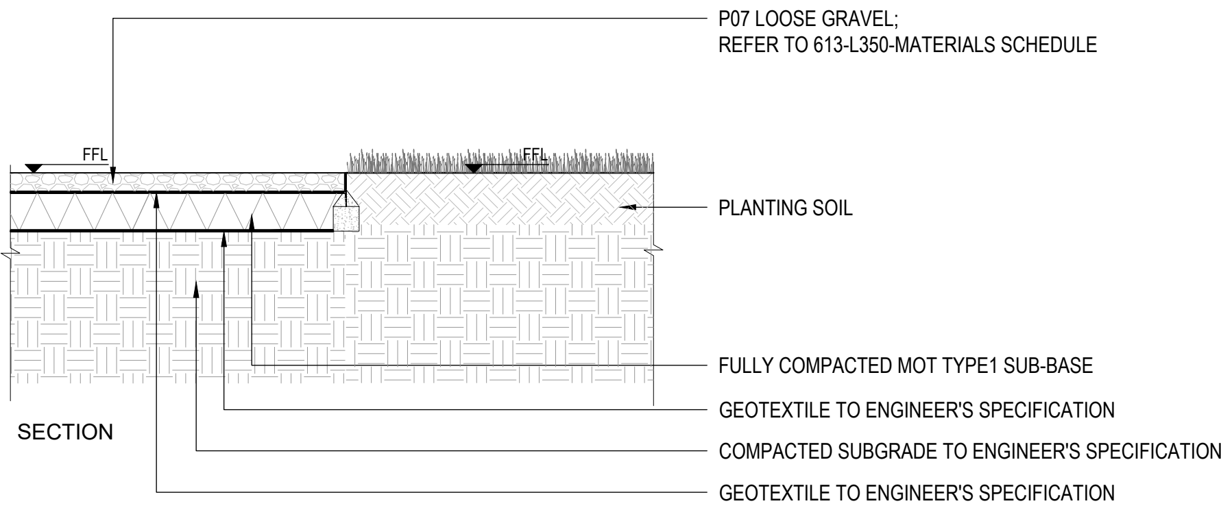
13 TYPICAL GRAVEL PATH AND PLANTING DETAIL SCALE : 1:20 @ A1
