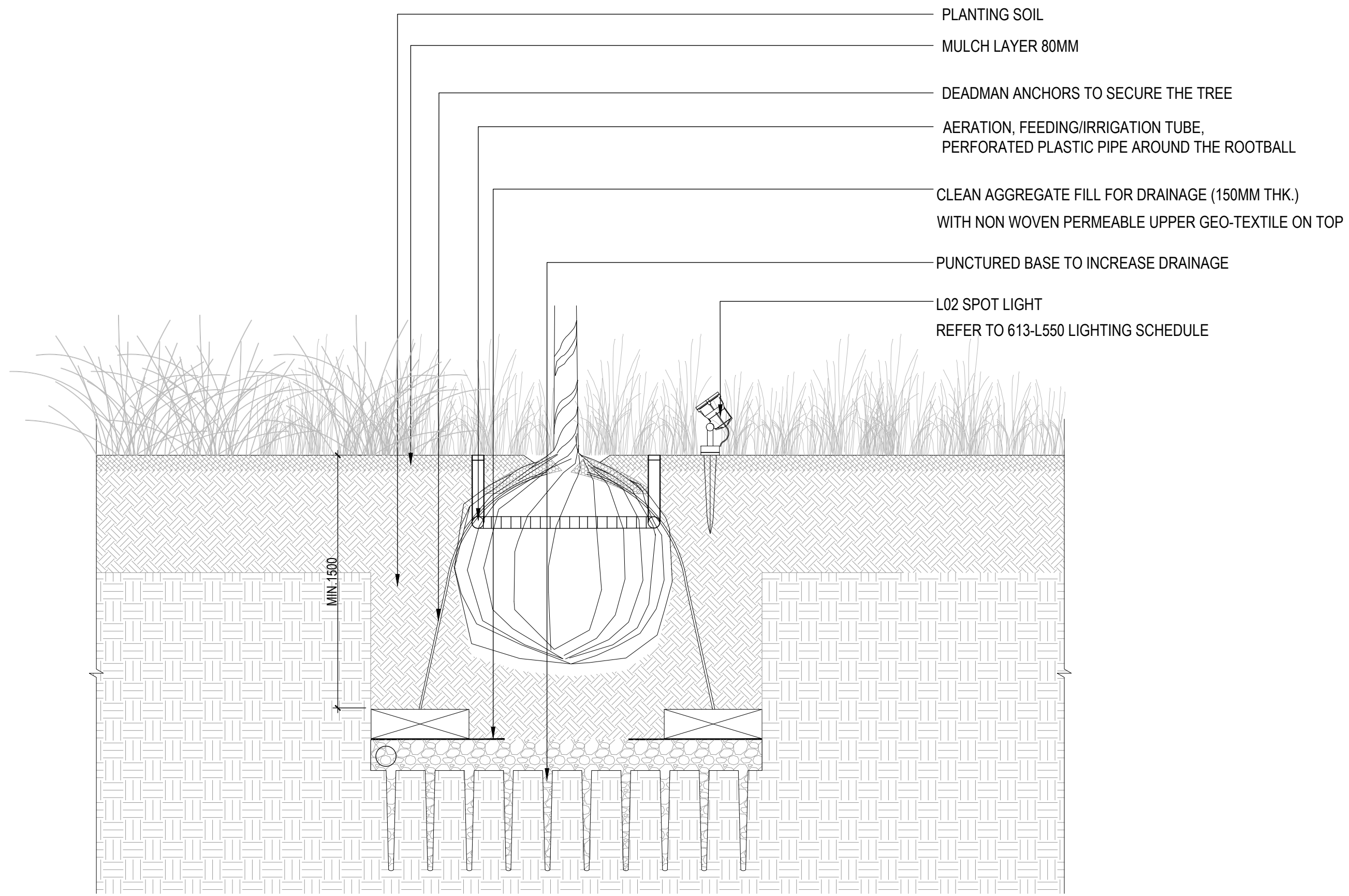
SECTION 16 TREE PIT WITH SHRUB-PLANTING ON GRADE (TYP.) SCALE : 1:20 @ A1
