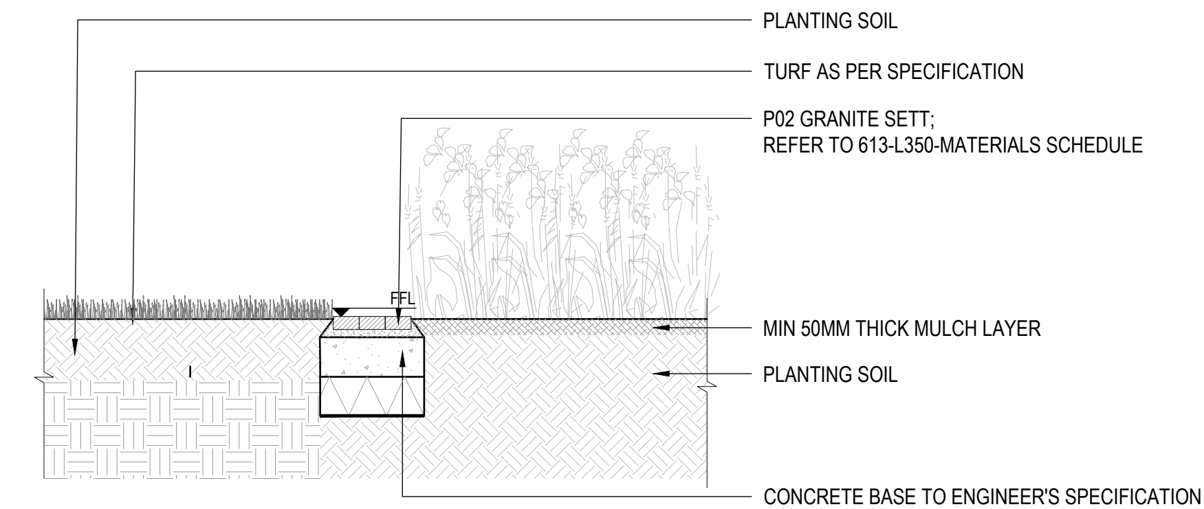
SECTION 09 TYPICAL SETT EDGE, TURF AND PLANTING DETAIL SCALE : 1:20 @ A1
