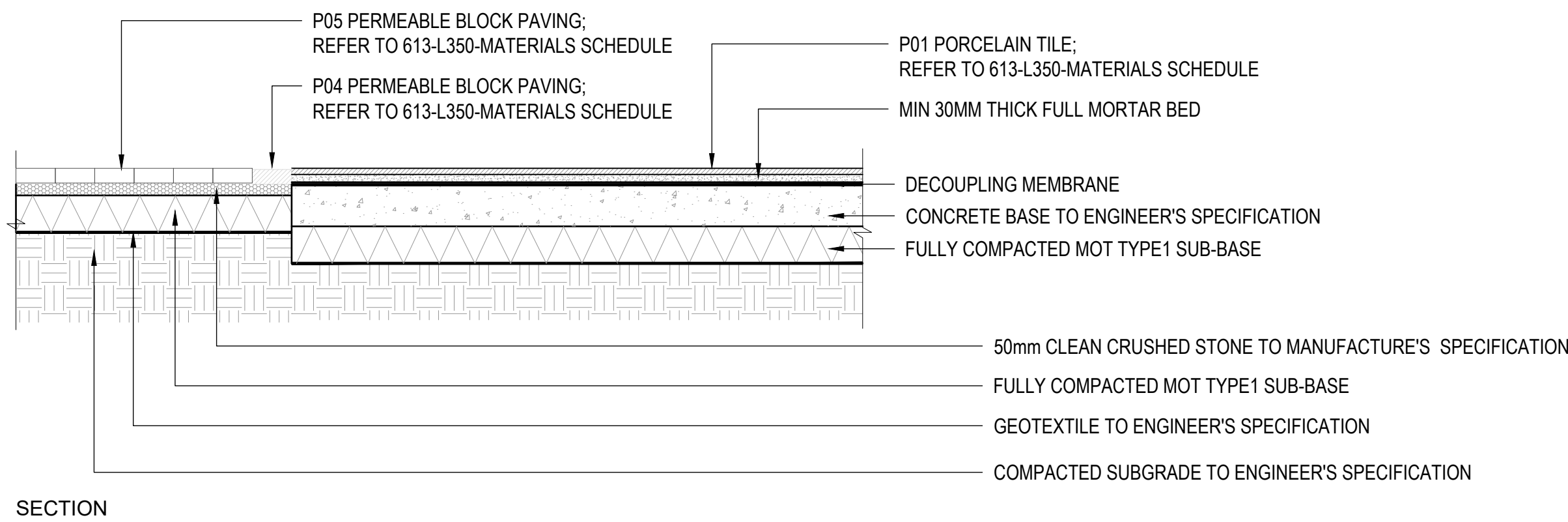
04 TYPICAL PERMEABLE BLOCK AND PORCELAIN TILE PAVING DETAIL SCALE : 1:20 @ A1
