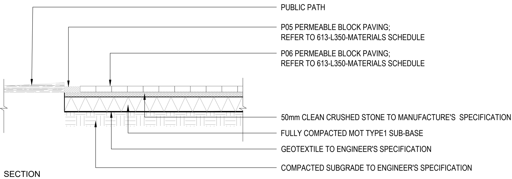
01 TYPICAL PERMEABLE BLOCK PAVING DETAIL SCALE : 1:20 @ A1
