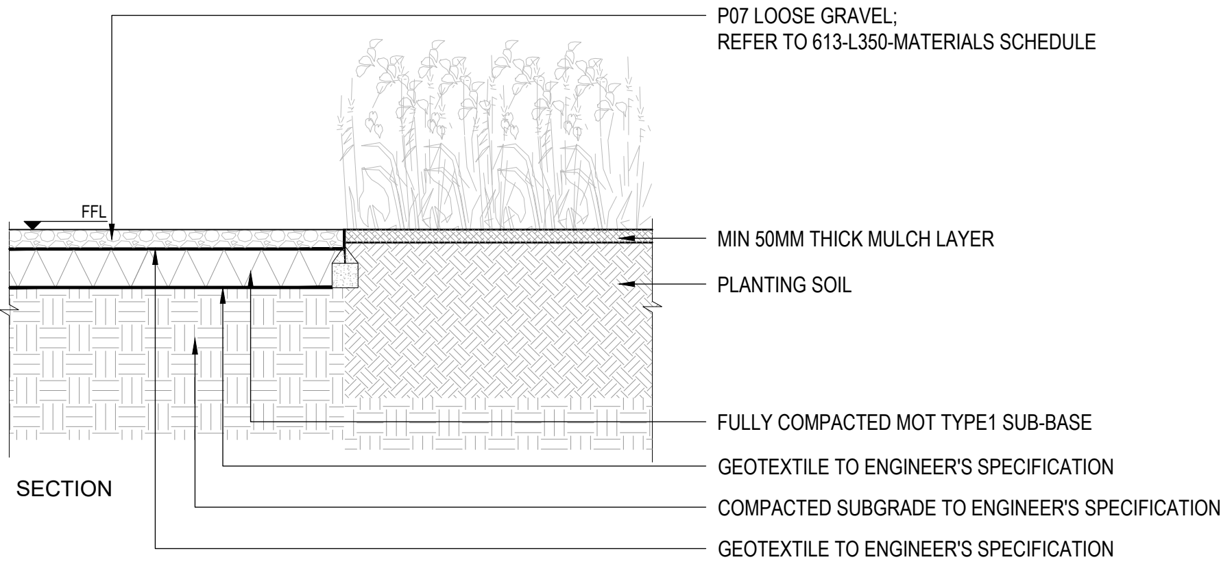
11 TYPICAL GRAVEL PATH AND PLANTING DETAIL SCALE : 1:20 @ A1
