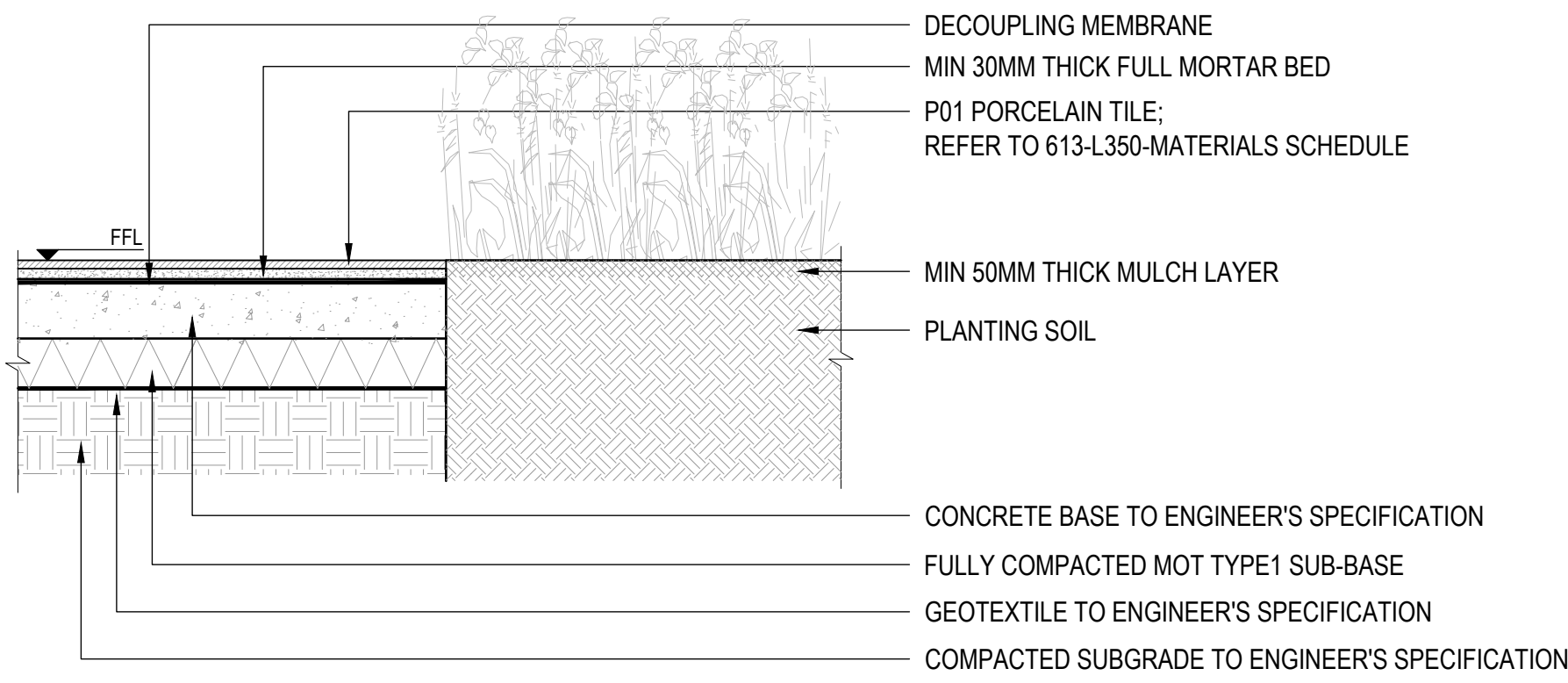
SECTION 06 TYPICAL PORCELAIN TILE PAVING AND PLANTING DETAIL SCALE: 1:20 @ A1
