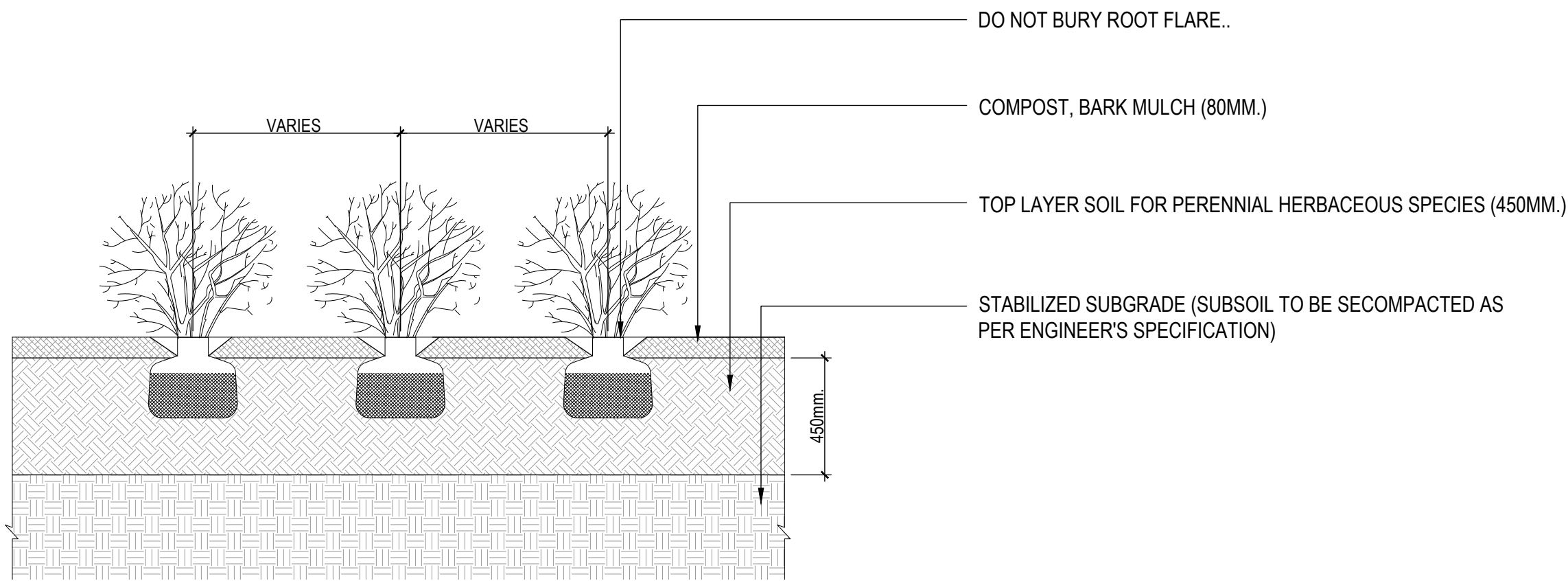
SECTION 15 PLANTER SHRUBS ON GRADE (TYP.) SCALE : 1:20 @ A1
