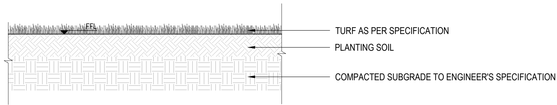
SECTION 14 TYPICAL TURF LAYING SCALE: 1:20 @ A1
