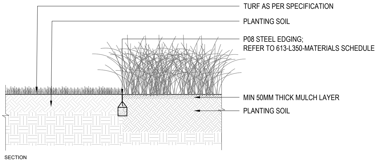
SECTION 07 TYPICAL PLANTING, STEEL EDGING AND TURF LAYING SCALE: 1:20 @ A1
