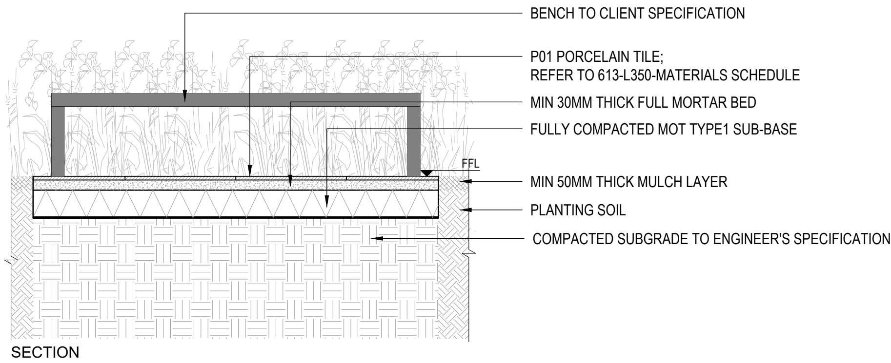
12 TYPICAL CONCRETE BASE AND BENCH DETAIL SCALE : 1:20 @ A1
