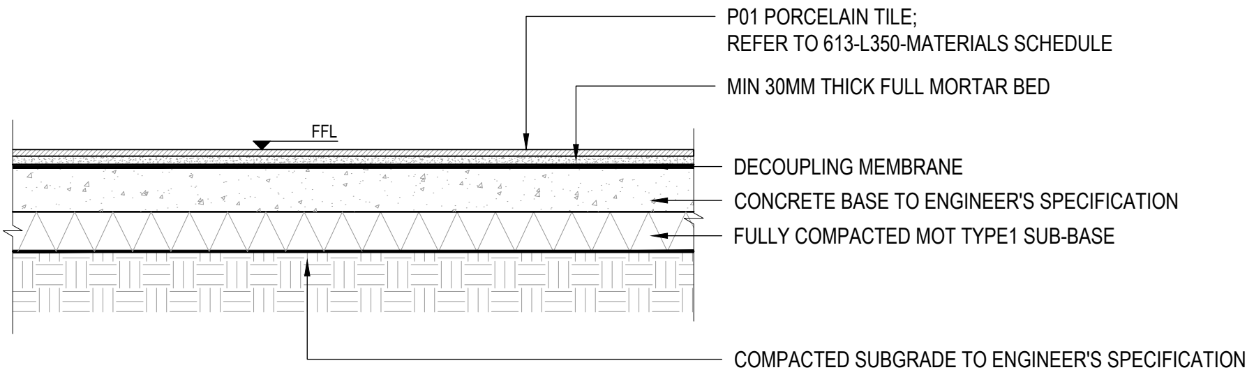
SECTION 05 TYPICAL PORCELAIN TILE PAVING DETAIL SCALE: 1:20 @ A1
