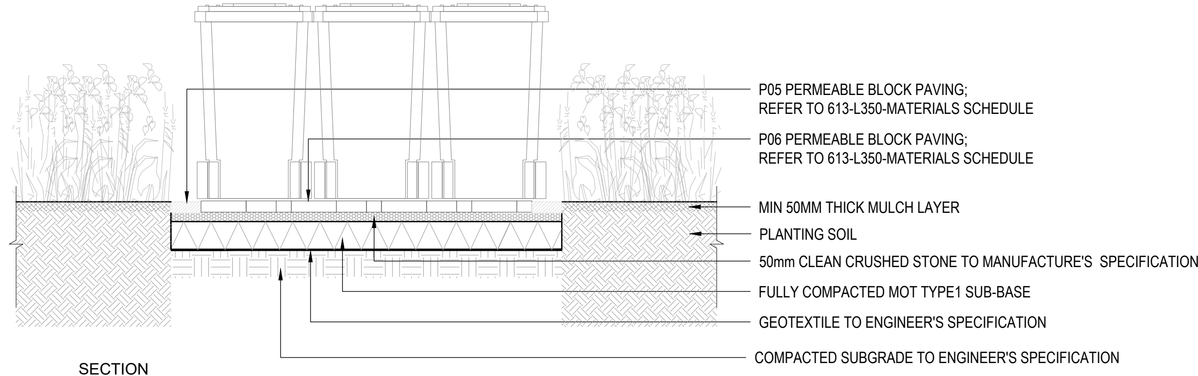
03 TYPICAL PERMEABLE BLOCK PAVING AND PLANTING DETAIL SCALE : 1:20 @ A1
