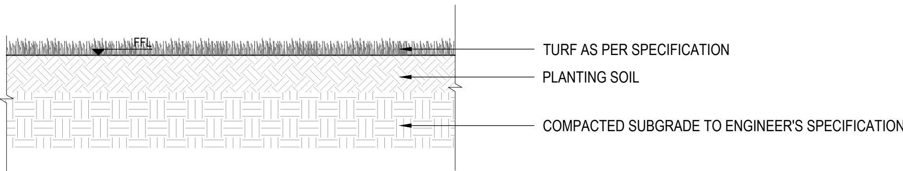
SECTION 14 TYPICAL TURF LAYING SCALE : 1:20 @ A1
