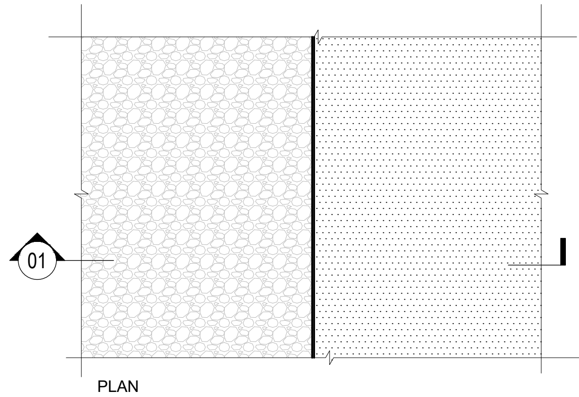
11 TYPICAL GRAVEL PATH AND PLANTING DETAIL SCALE : 1:20 @ A1
