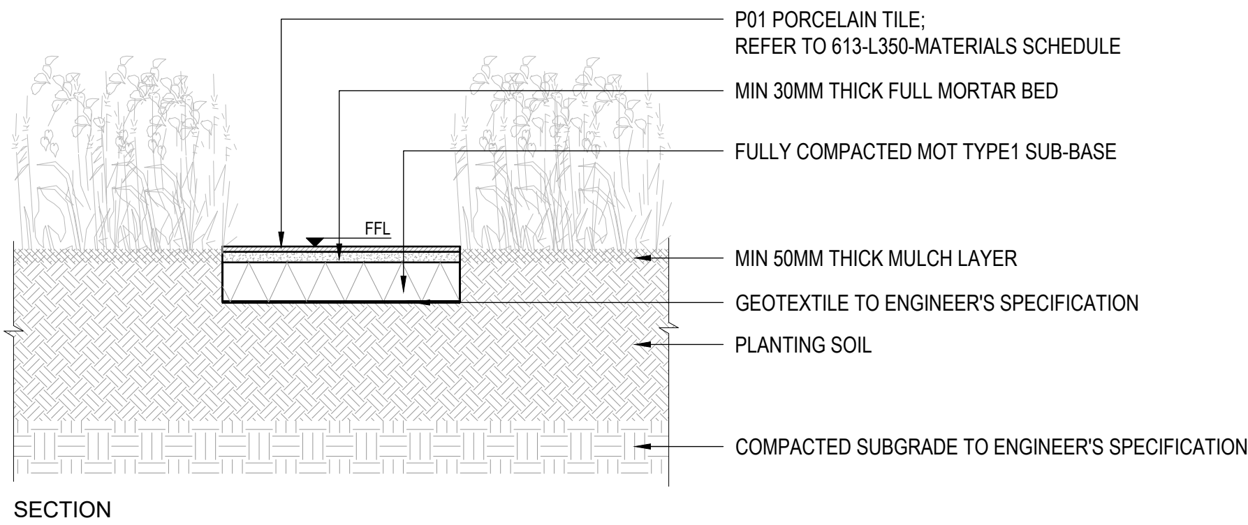
10 TYPICAL STEPPING STONE IN PLANTING AREA DETAIL SCALE : 1:20 @ A1
