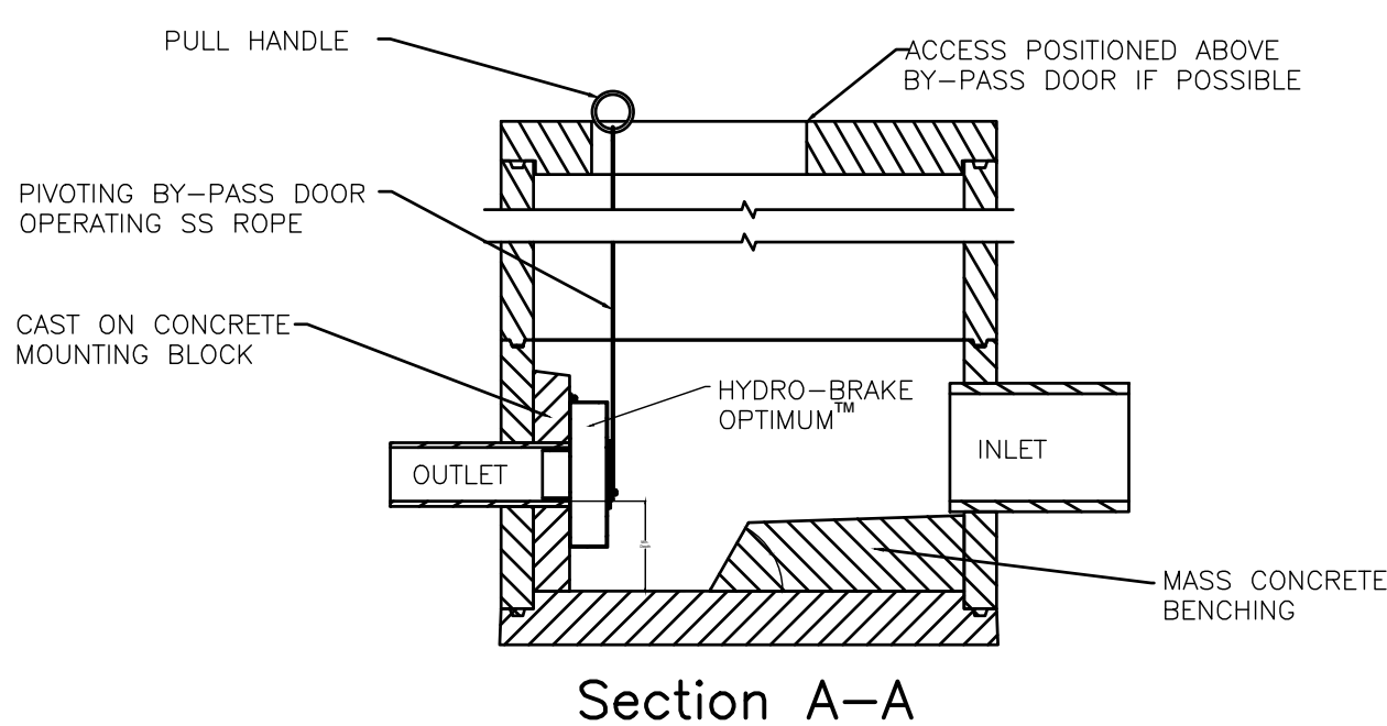
HYDROBRAKE MANHOLE
