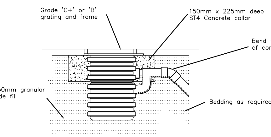
YARD GULLY DETAIL
