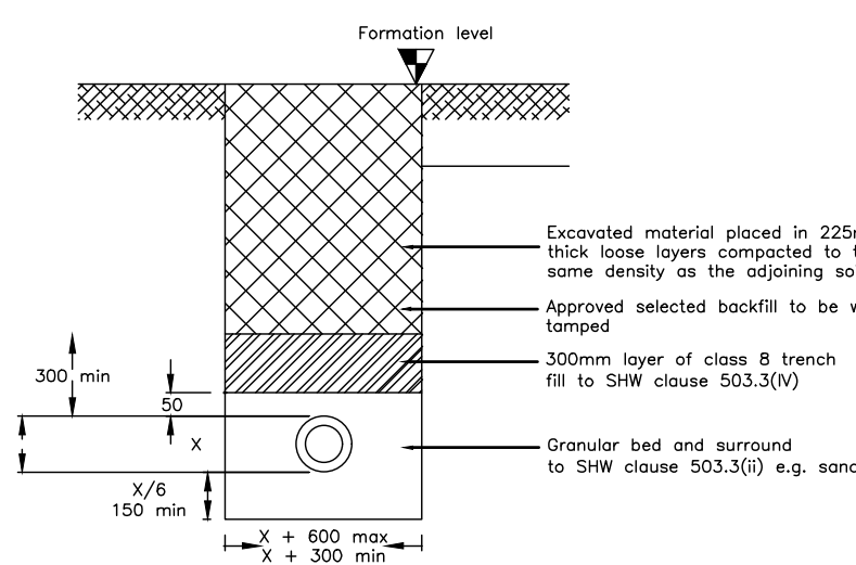
TYPE T PIPE BEDDING IN VERGES AND OTHER UNTRAFFICKED AREAS
