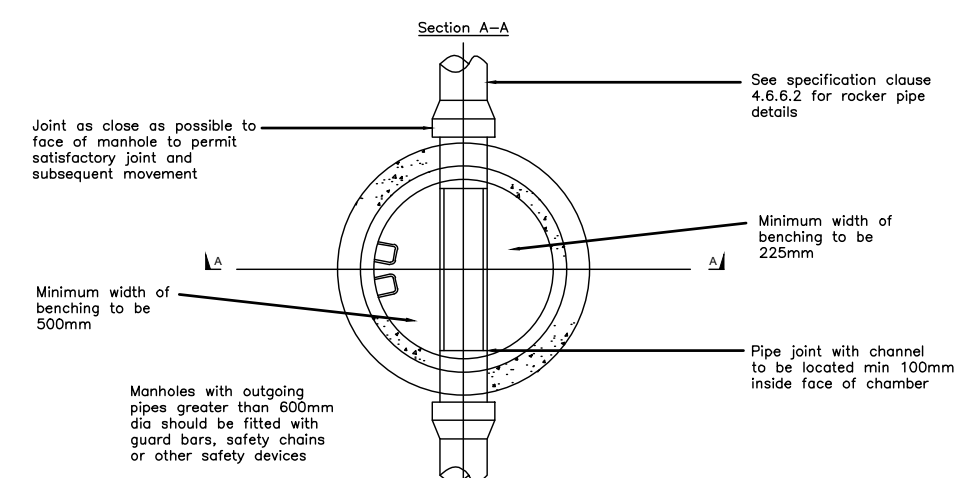
TYPICAL MANHOLE – Type 2 Max depth from ground level to soffit of pipe 3.0m
