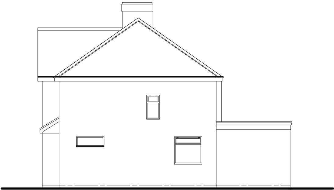
SIDE ELEVATION
