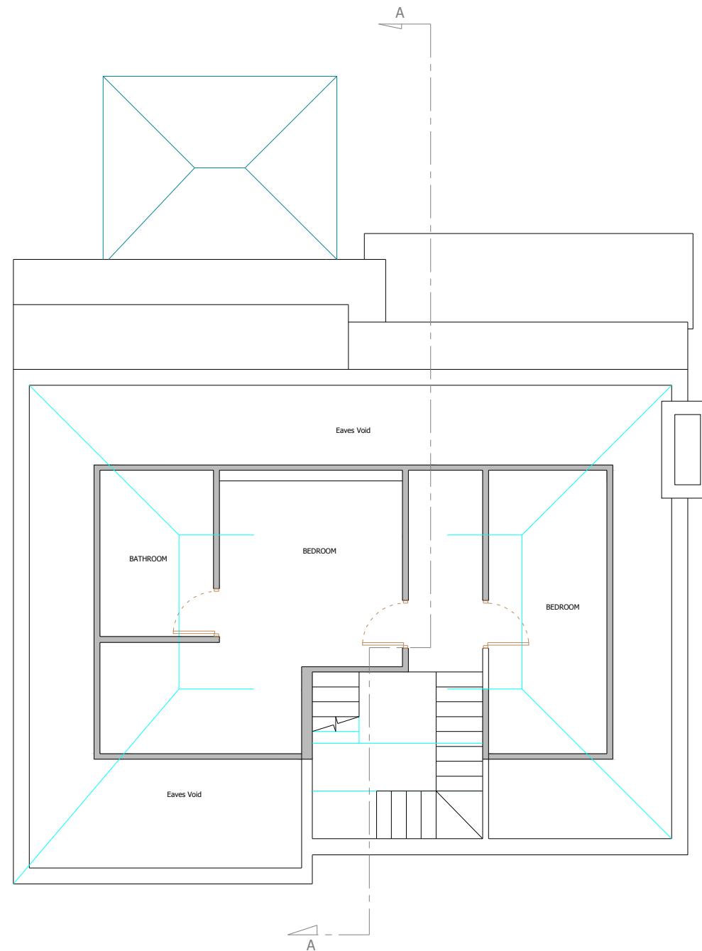
7 LOFT EXISTING PLAN
