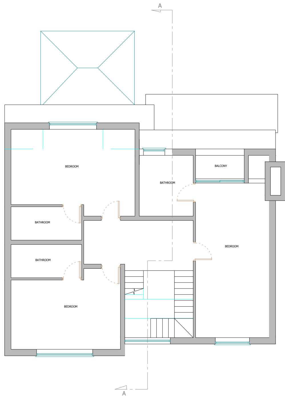
6 FIRST FLOOR EXISTING PLAN
