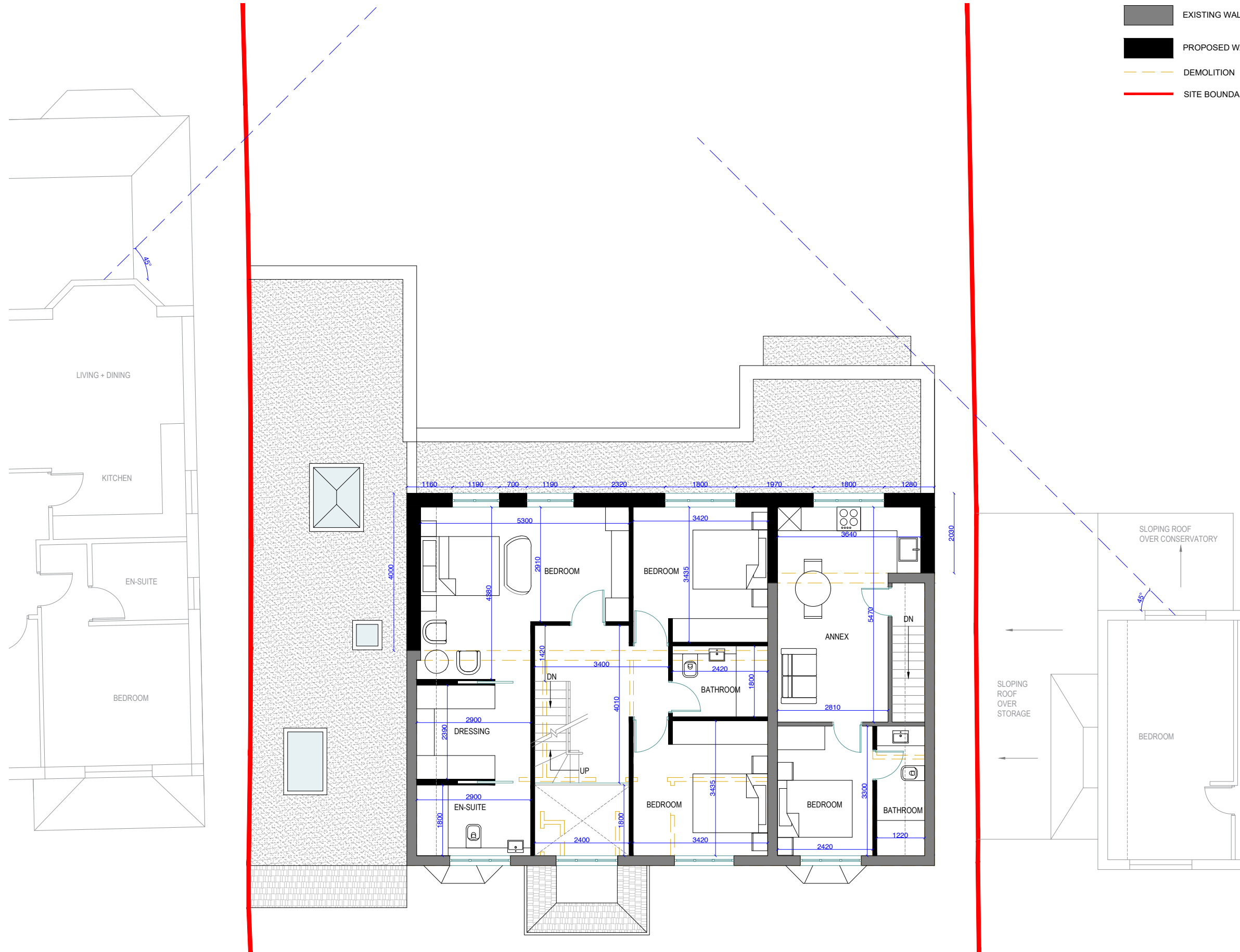
1 PROPOSED FIRST FLOOR PLAN
