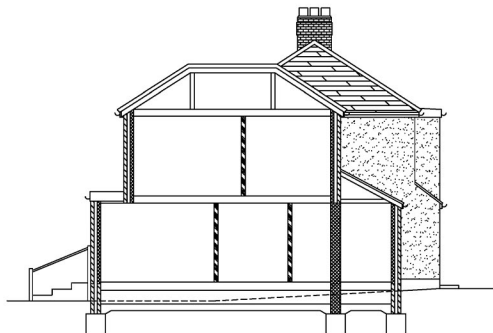
PROPOSED SECTION
