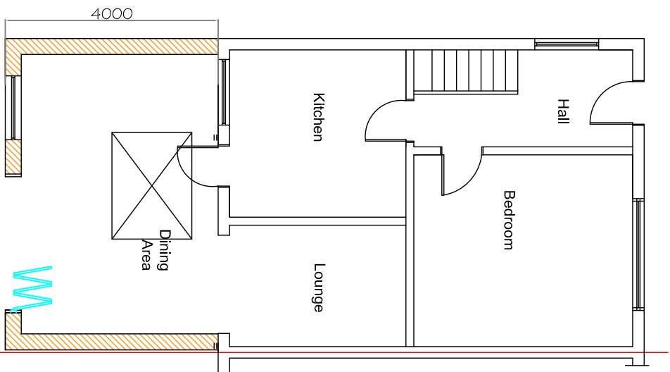
Proposed Ground Floor Plan 1;100
