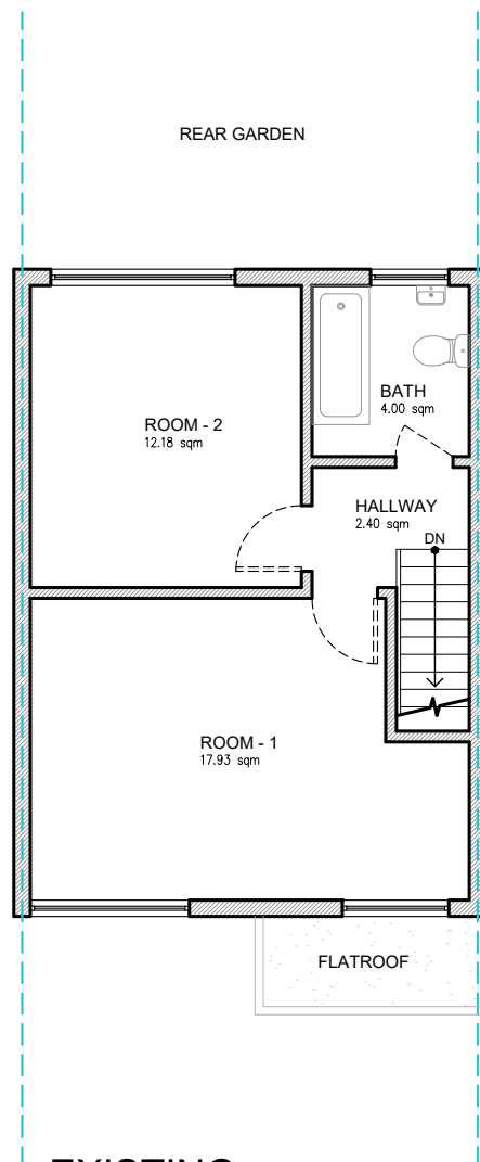
EXISTING FIRST FLOOR GIA = 40.15 M 2
