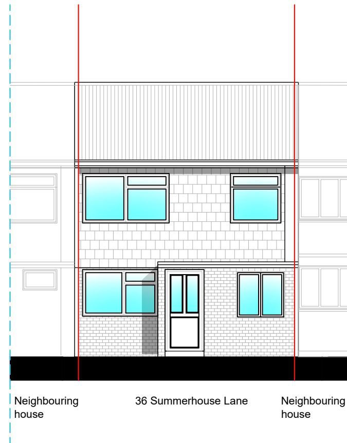
NORTH-EAST ELEVATION (FRONT VIEW)
