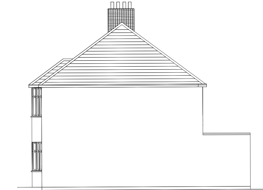
PROPOSED SIDE ELEVATION(FROM NO.23)
