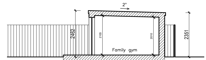
PROPOSED SECTION
