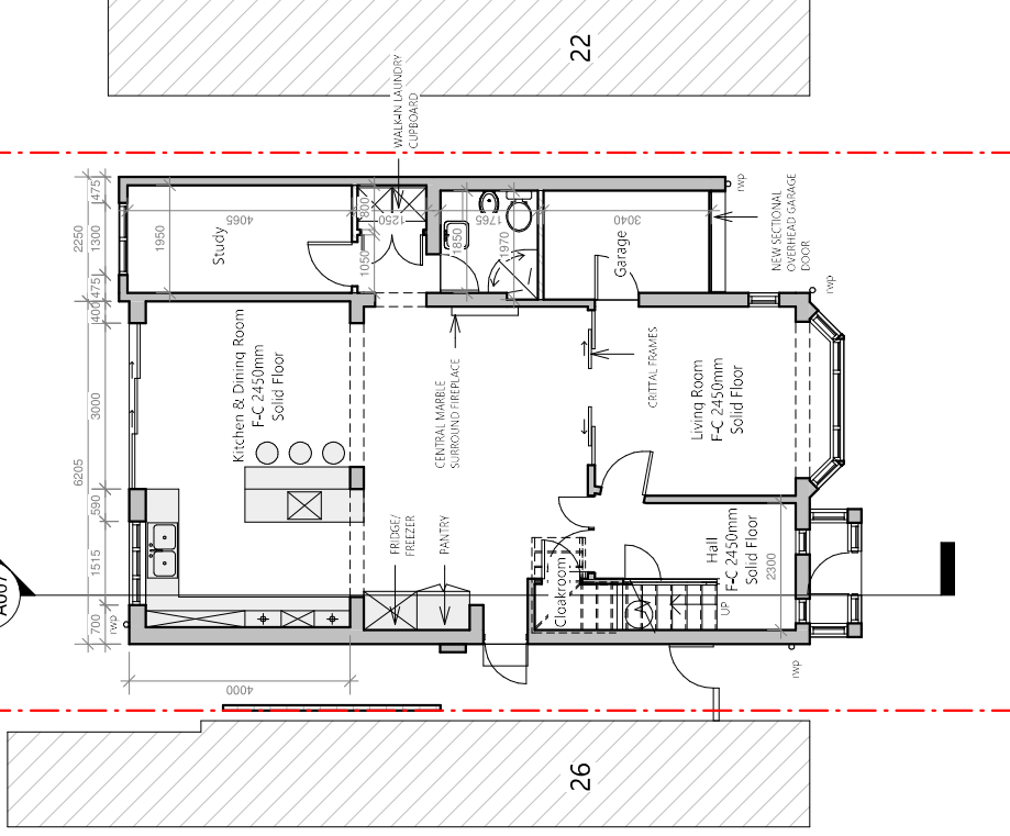
2 Proposed Ground Floor 1 : 100
