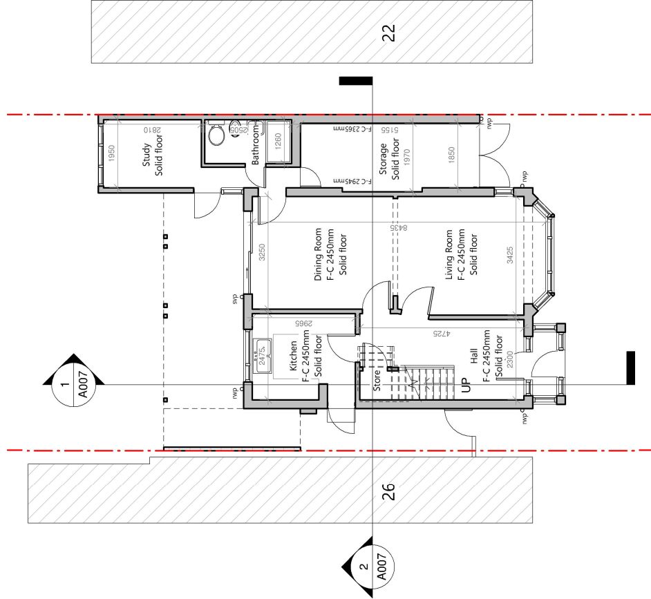
1 Existing Ground Floor 1 : 100
