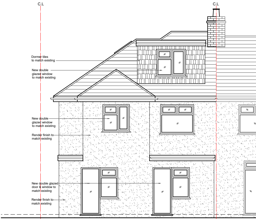
02 - REAR ELEVATION
