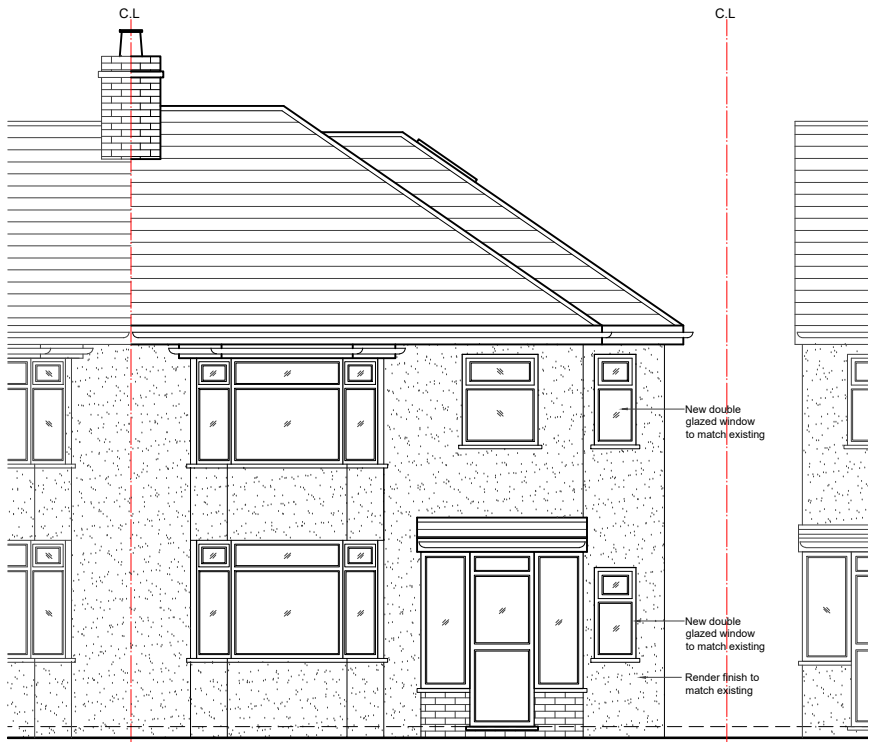
01 - FRONT ELEVATION
