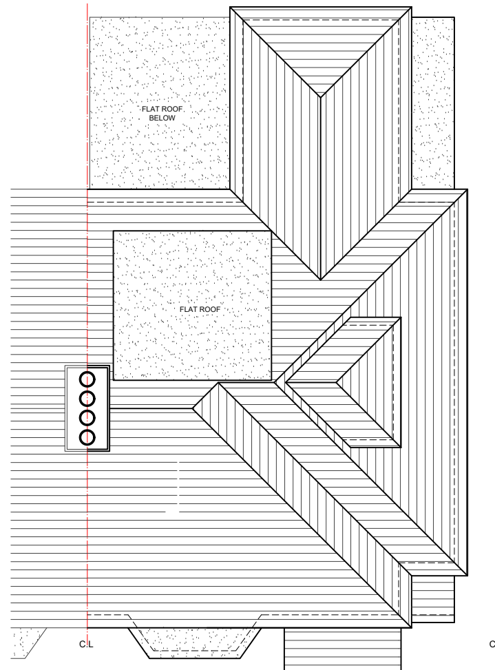
04 - ROOF PLAN
