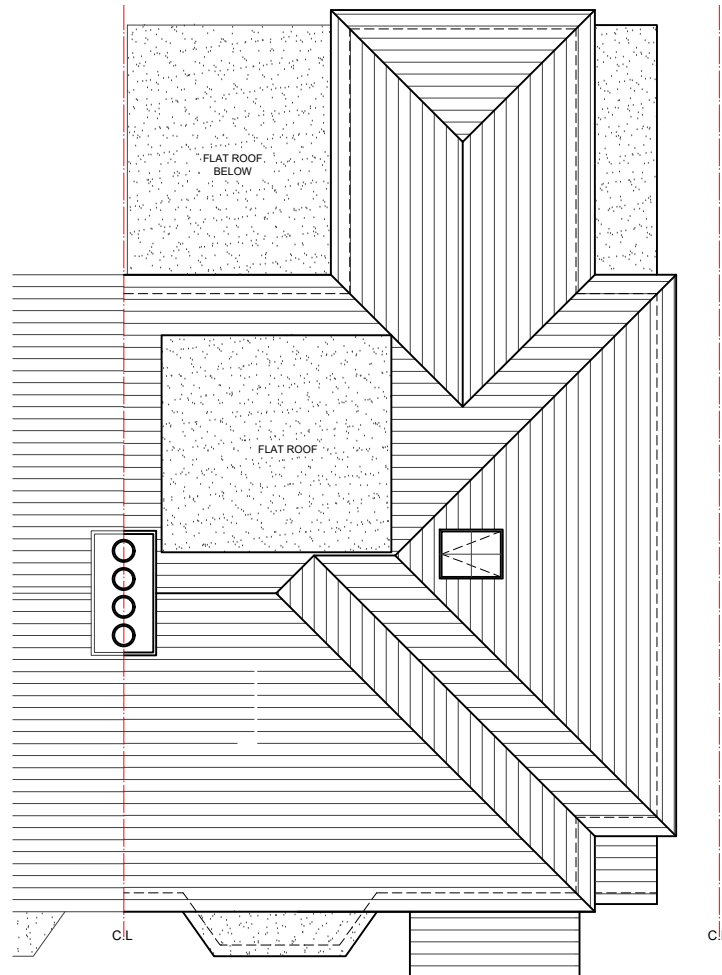
04 - ROOF PLAN
