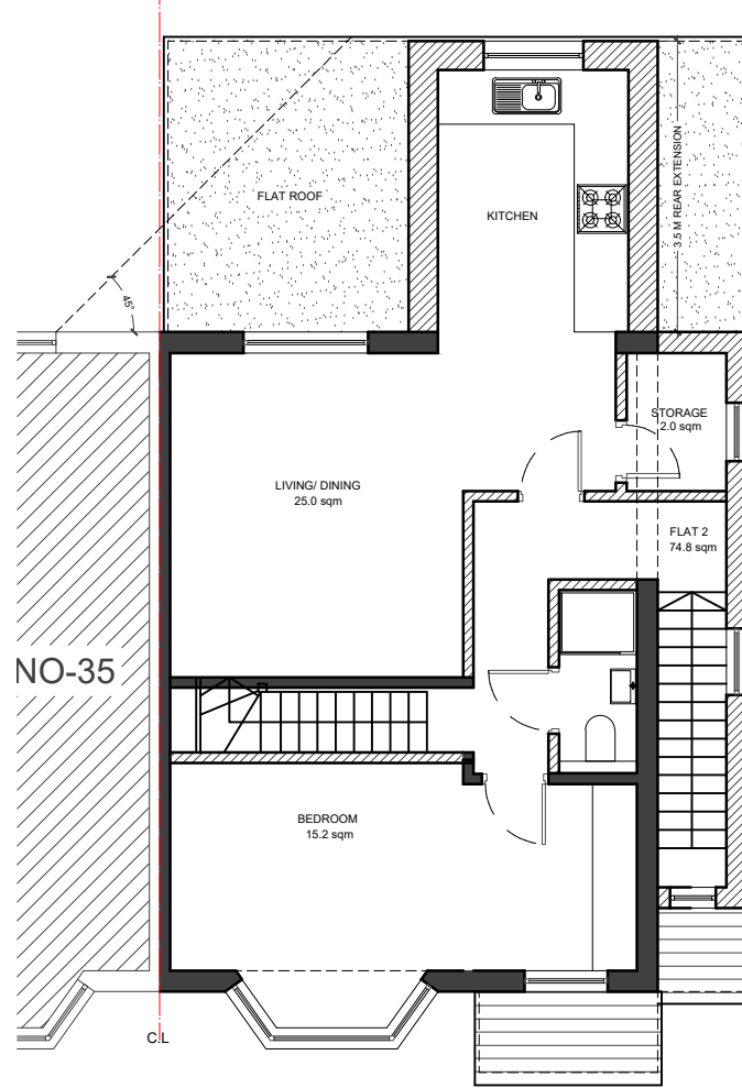
02 - FIRST FLOOR PLAN
