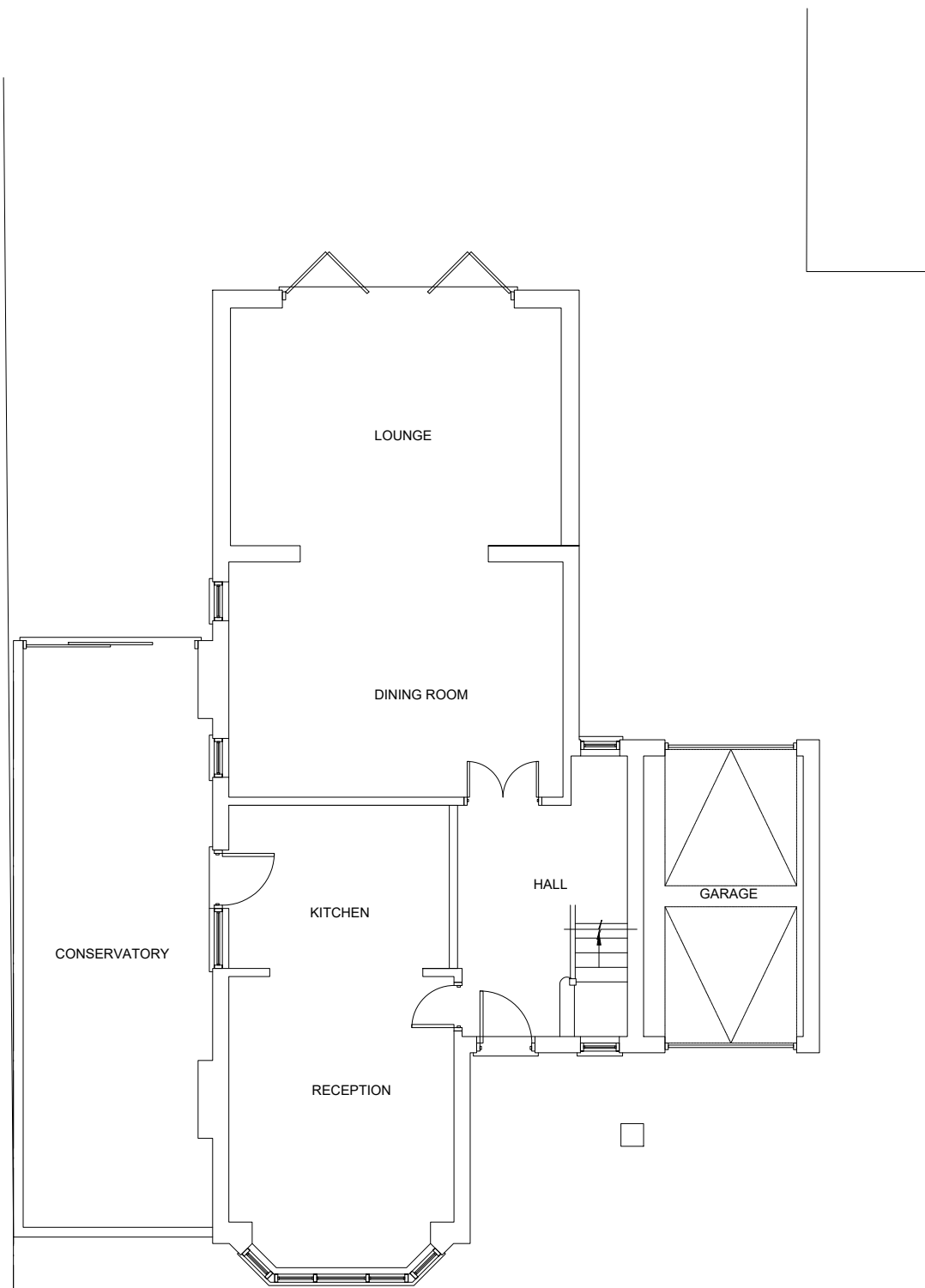
Pre Existing Ground Floor Plan
