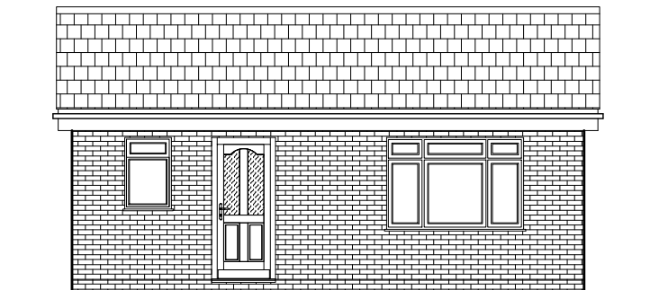
Front Elevation Scale 1:100
