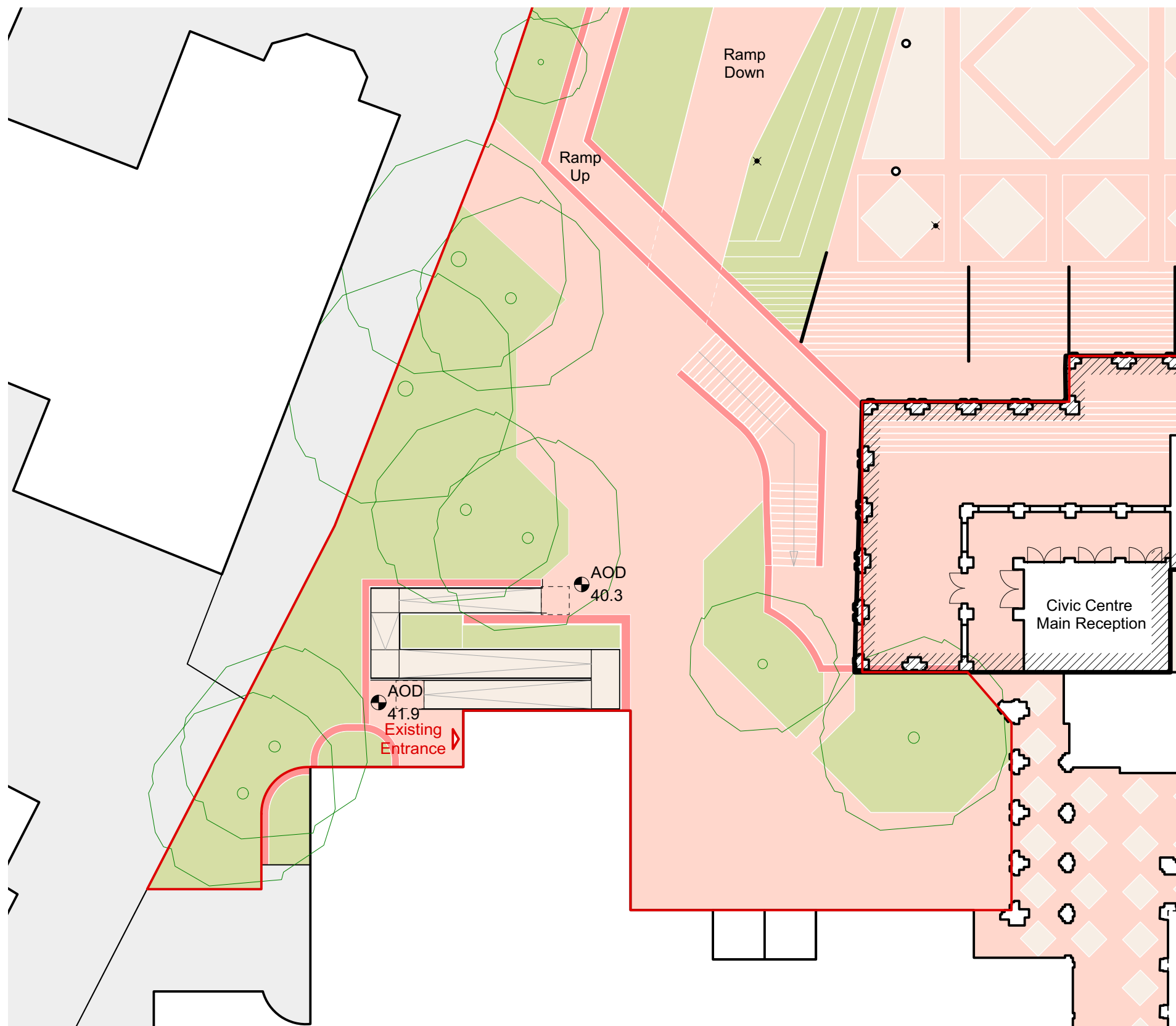
1 Proposed Ramp Design - Location Plan Scale: 1:250 @ A3
