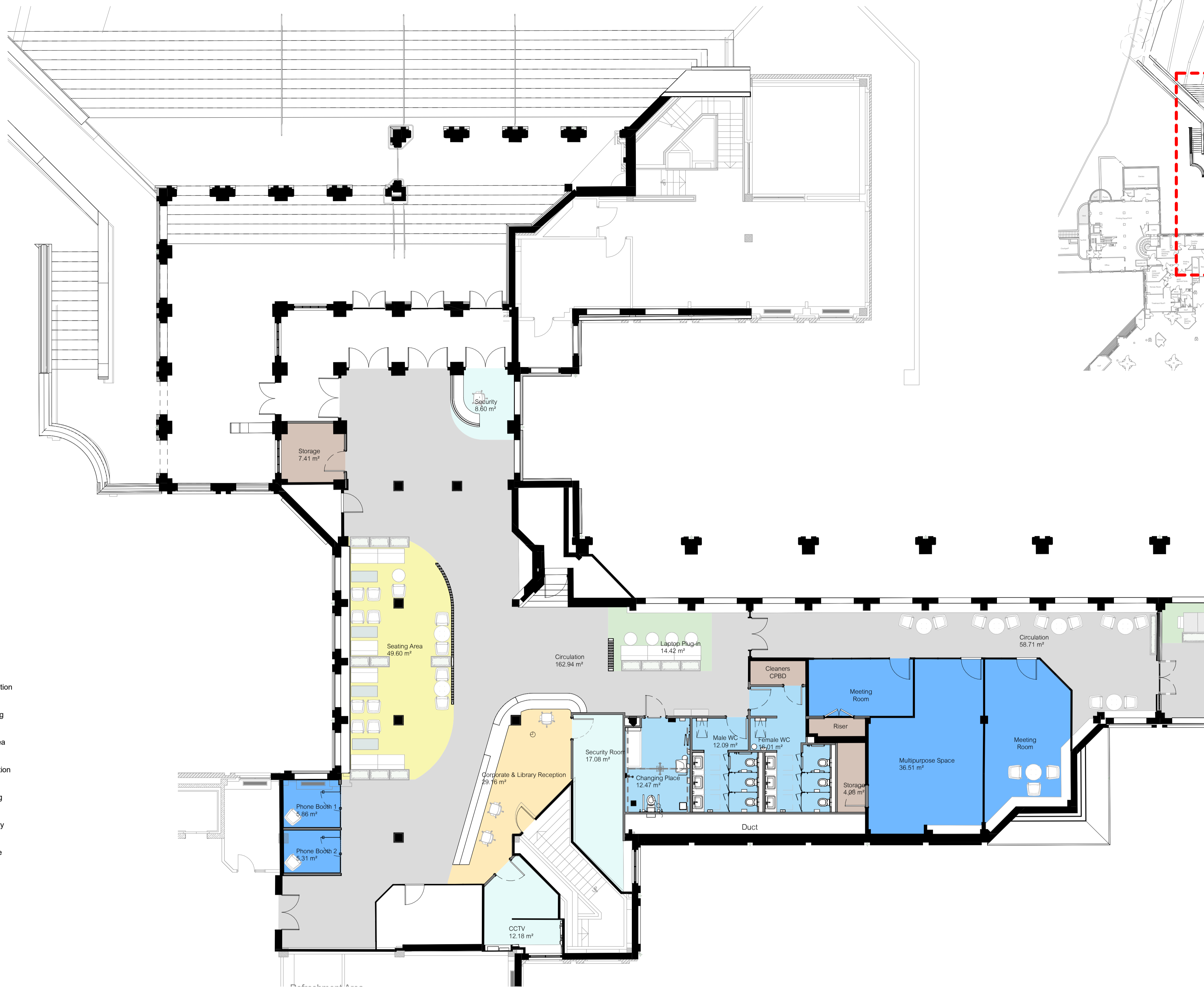
01 Level 2 - Entrance Proposed Plan 1 : 100
