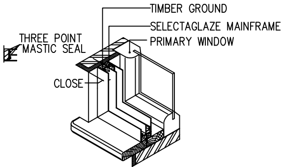
INSTALLATION DETAIL
