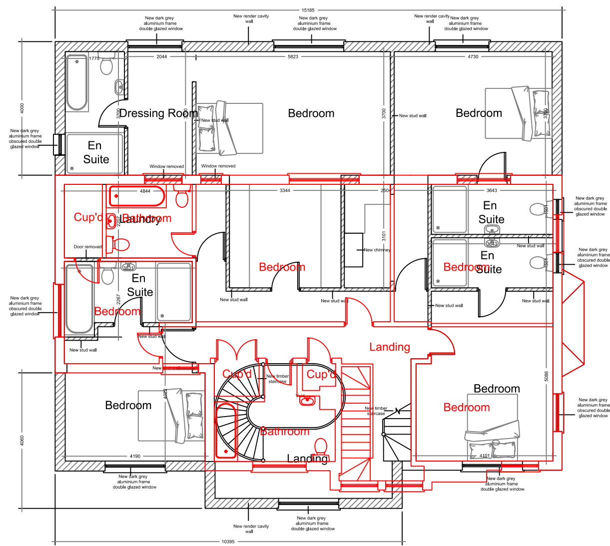
Existing First Floor Plan Proposed First Floor Plan
