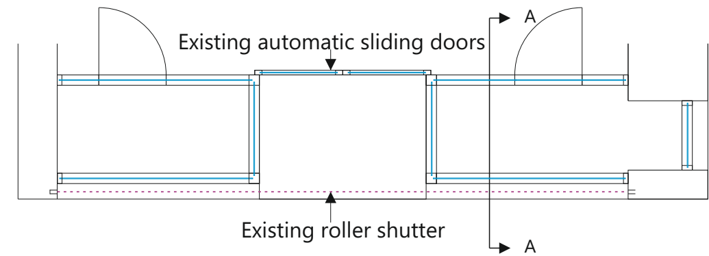
SHOPFRONT PLAN
