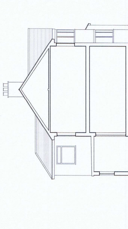
Existing section A-A
