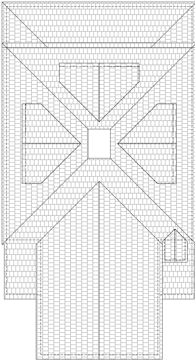
ROOF PLAN
