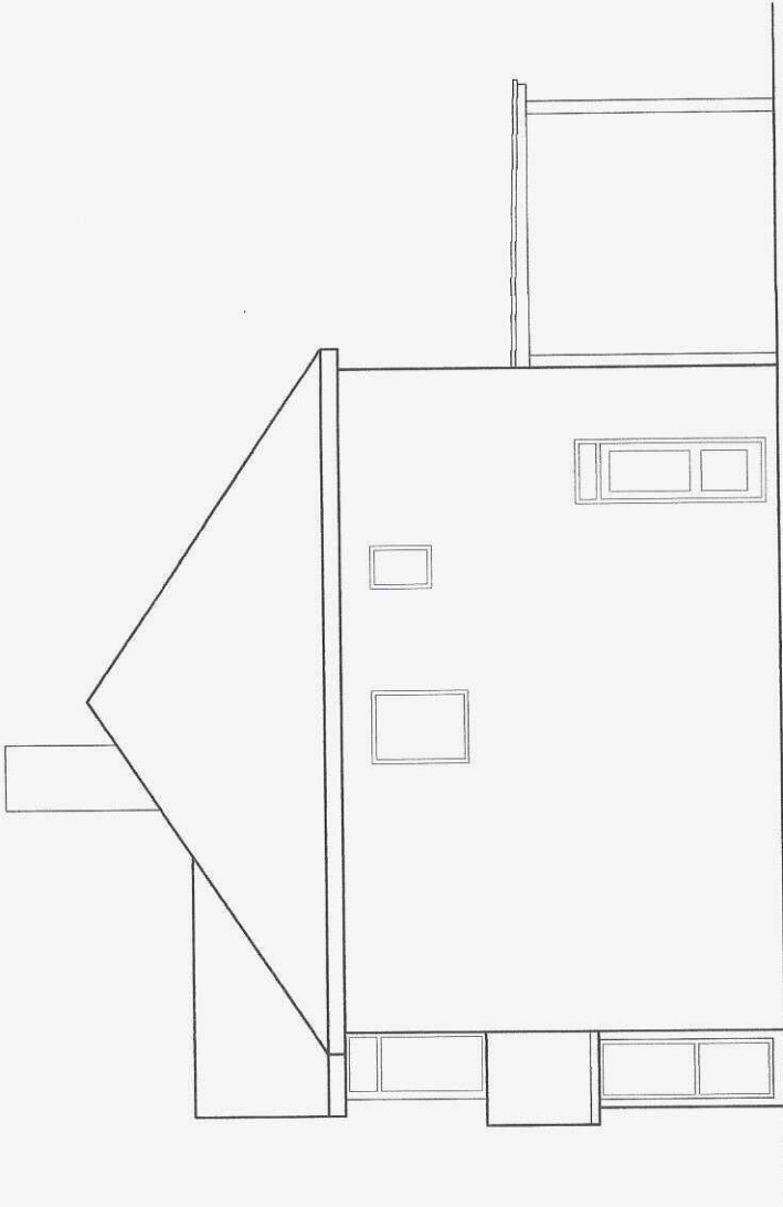
EXISTING R SIDE ELEVATION SCALE 1 : 100
