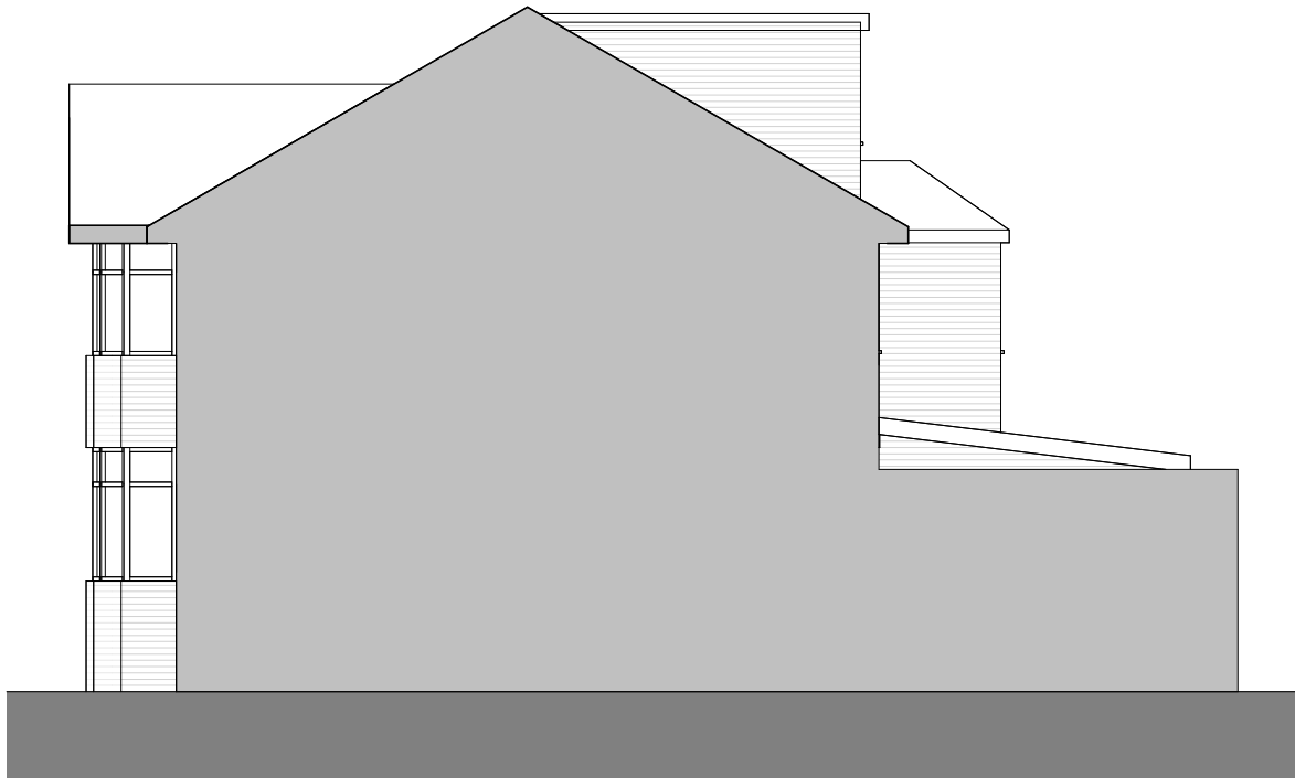
1 Proposed Side Elevation Scale - 1 : 100
