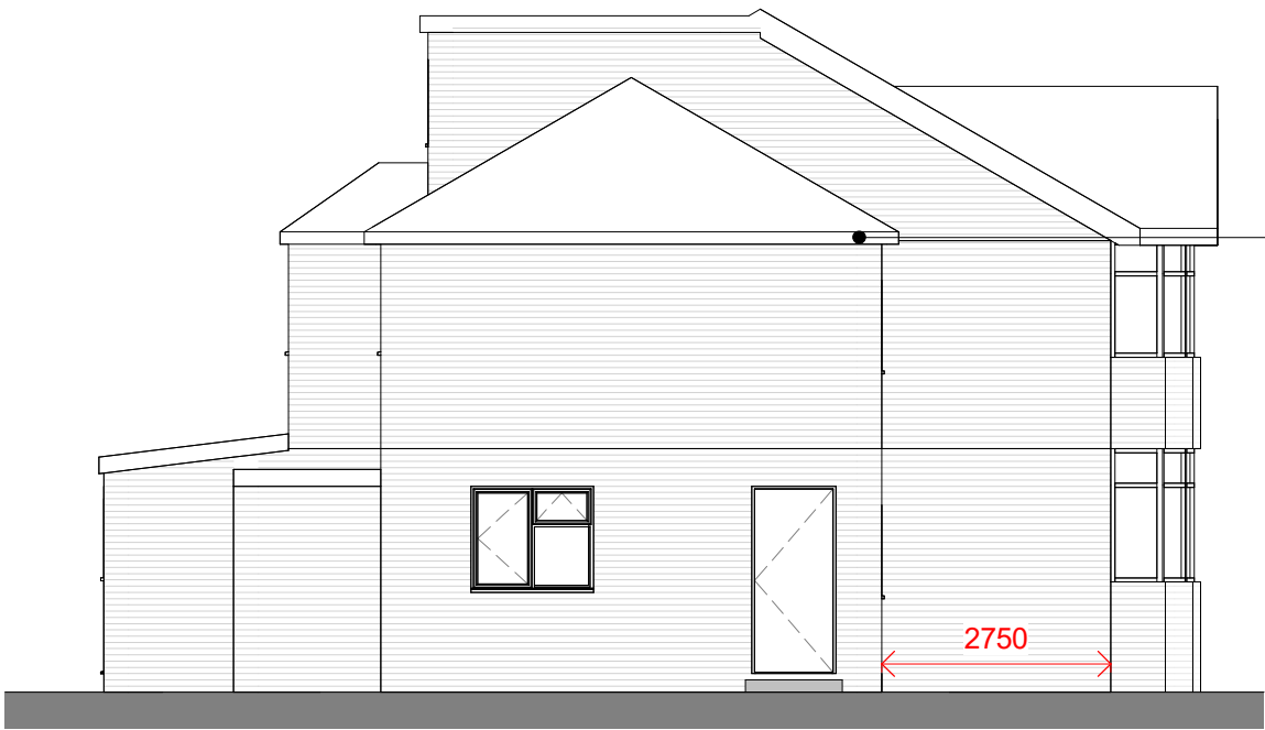
2 Proposed Side Elevation Scale - 1 : 100
