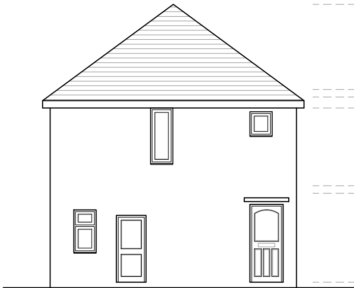
EXISTING NORTH SIDE ELEVATION SCALE= 1:100
