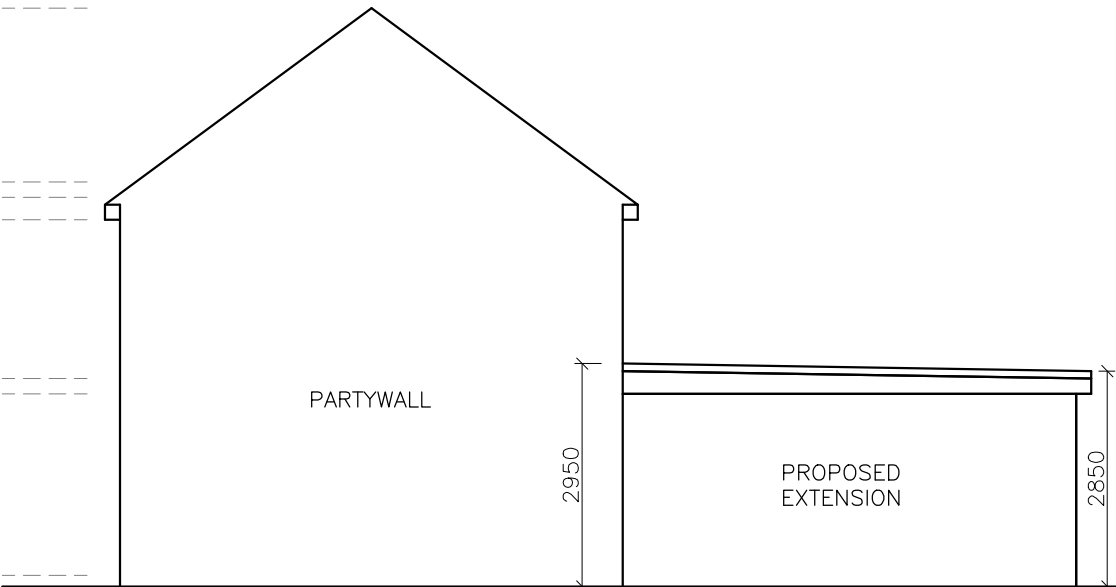
PROPOSED SOUTH SIDE ELEVATION SCALE= 1:100
