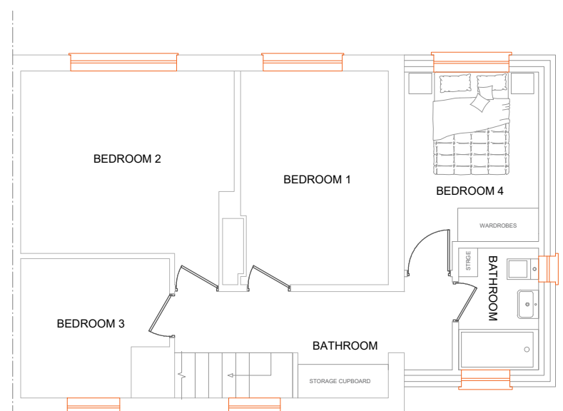
PROPOSED 1ST FLOOR PLAN
