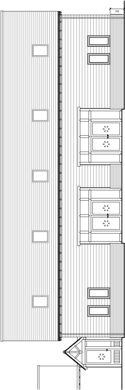
North West Elevation: Proposed
