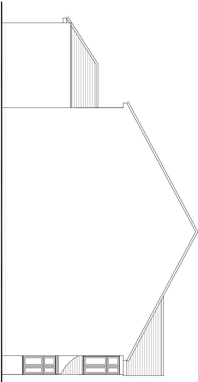
SIDE ELEVATION
