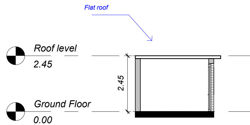
Proposed Section
