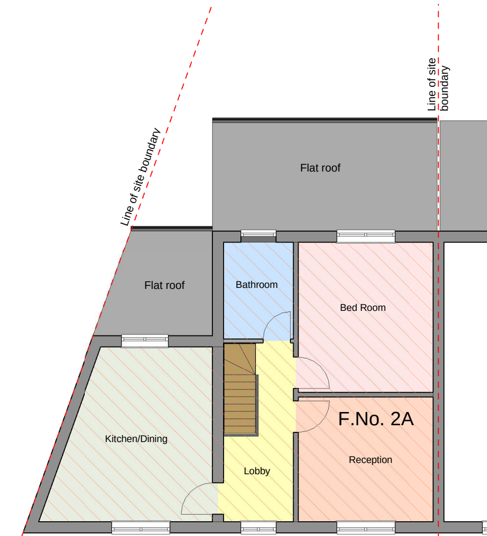
2 First Floor 03-A-301 1 : 100
