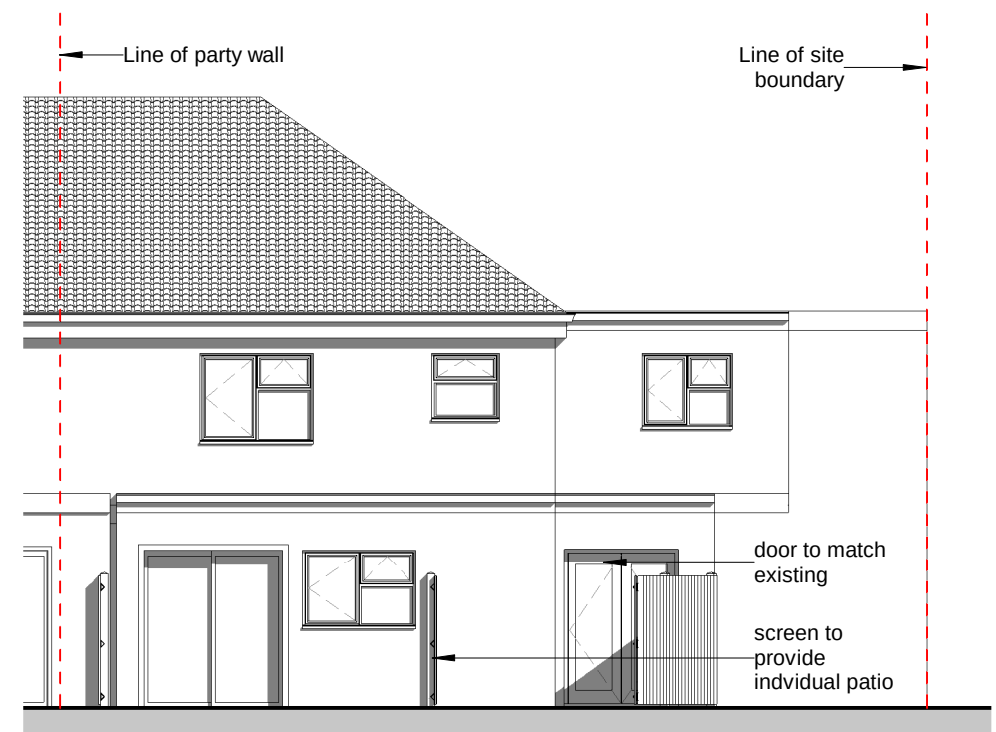
5 Rear Elevation 03-A-301 1 : 100
