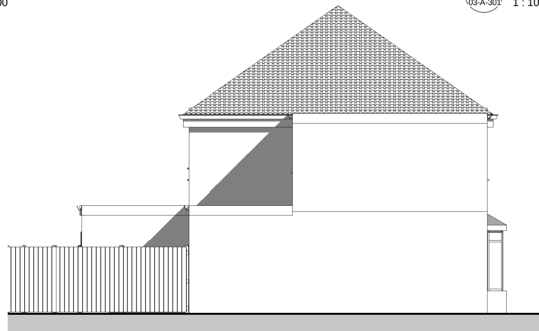
4 Side Elevation (Proposed) 03-A-301 1 : 100
