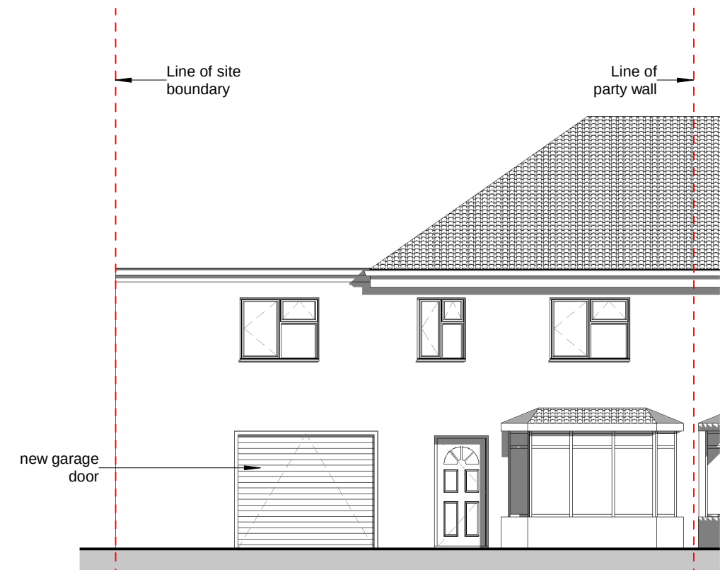
3 Front Elevation 03-A-301 1 : 100
