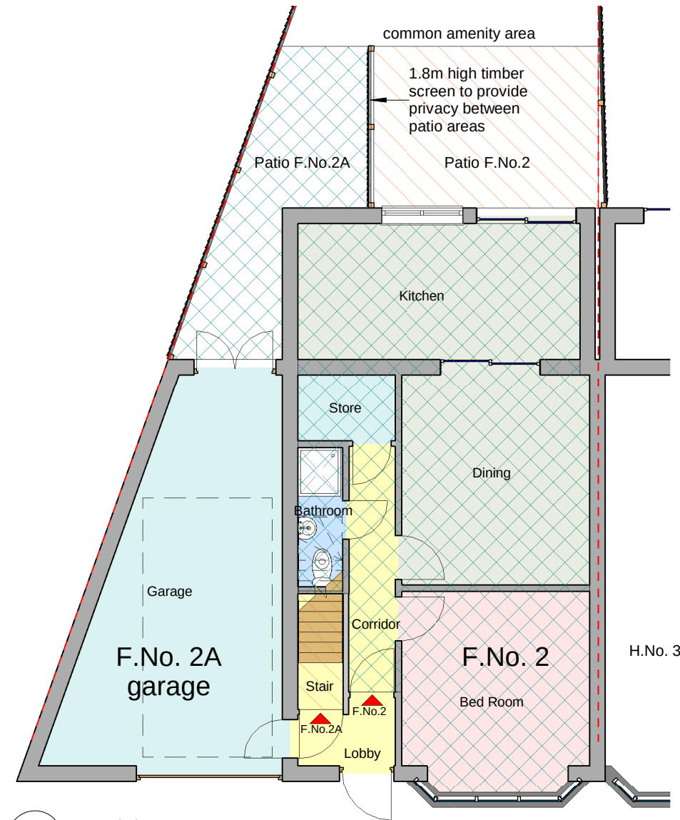
1 Ground Floor 03-A-301 1 : 100
